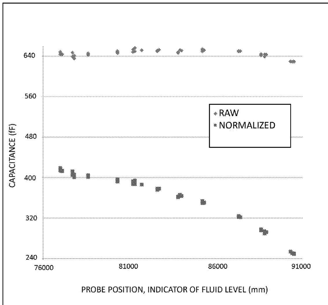
FIG. 9 PROBE POSITION VERSUS CAPACITANCE
