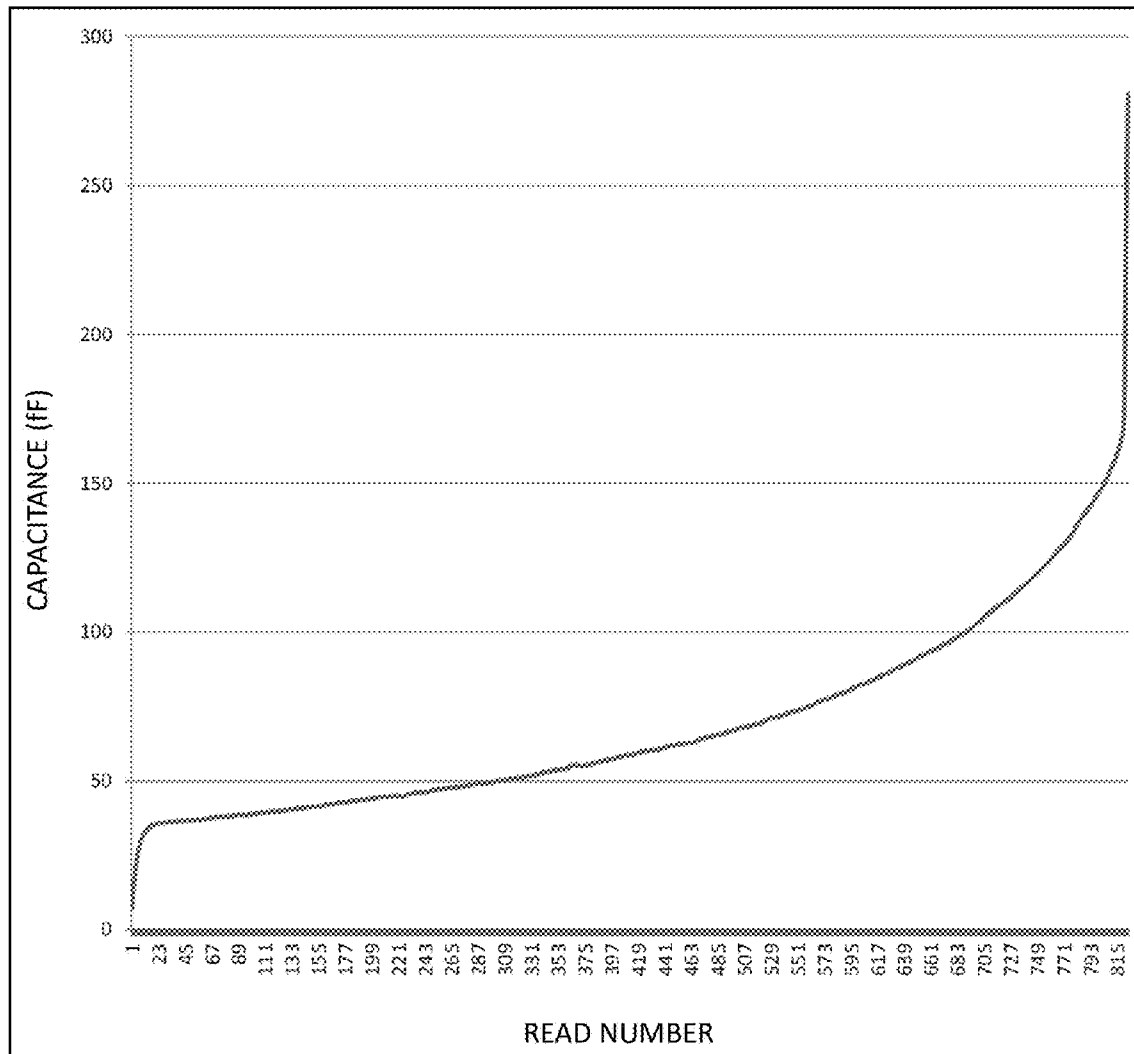
FIG. 8 READ NUMBER VERSUS CAPACITANCE APPROACH PLOT
