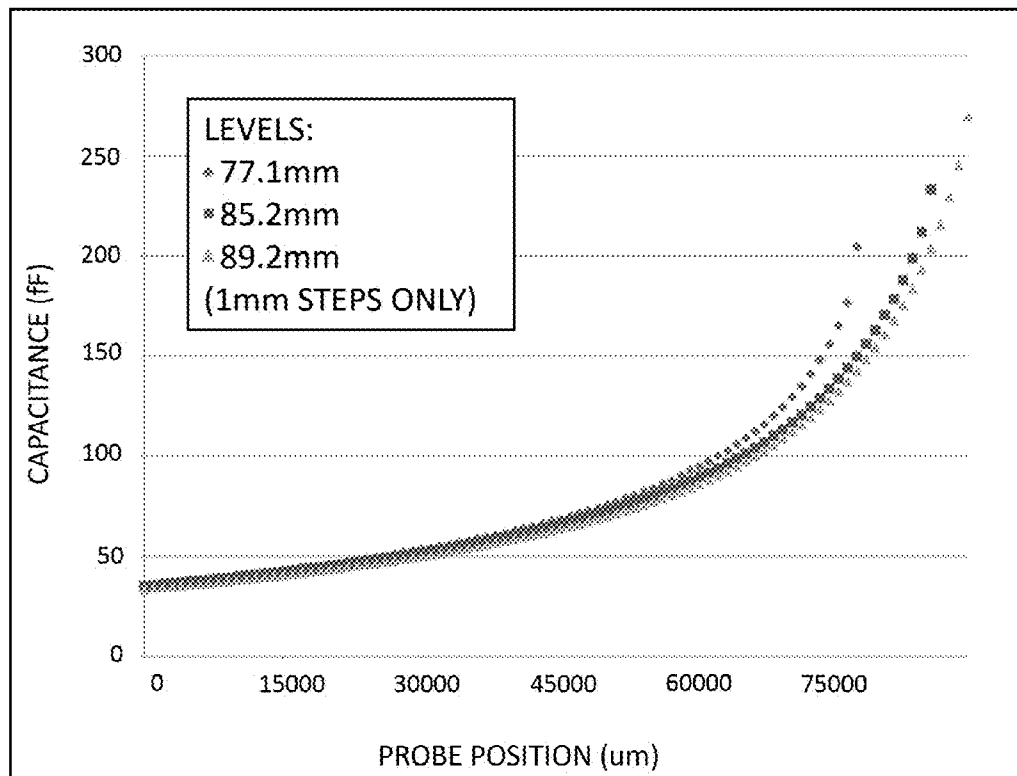
FIG. 5 CAPACITANCE VERSUS DISTANCE (AND FILL LEVEL)
