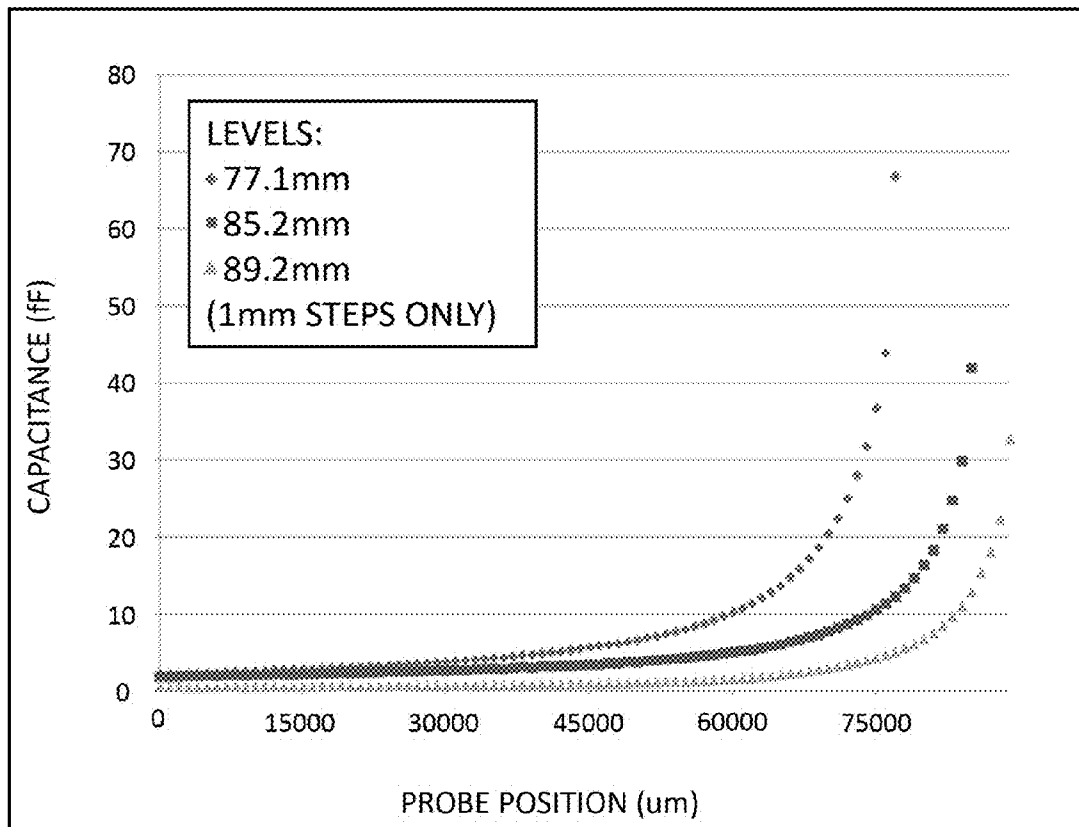
FIG. 6 NORMALIZED CAPACITANCE VERSUS DISTANCE (AND FILL LEVEL)
