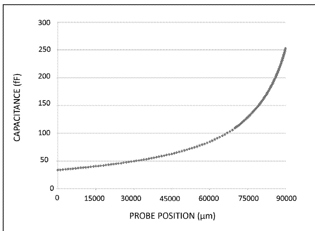
FIG. 3 BASELINE DATA – EMPTY CUVETTE
