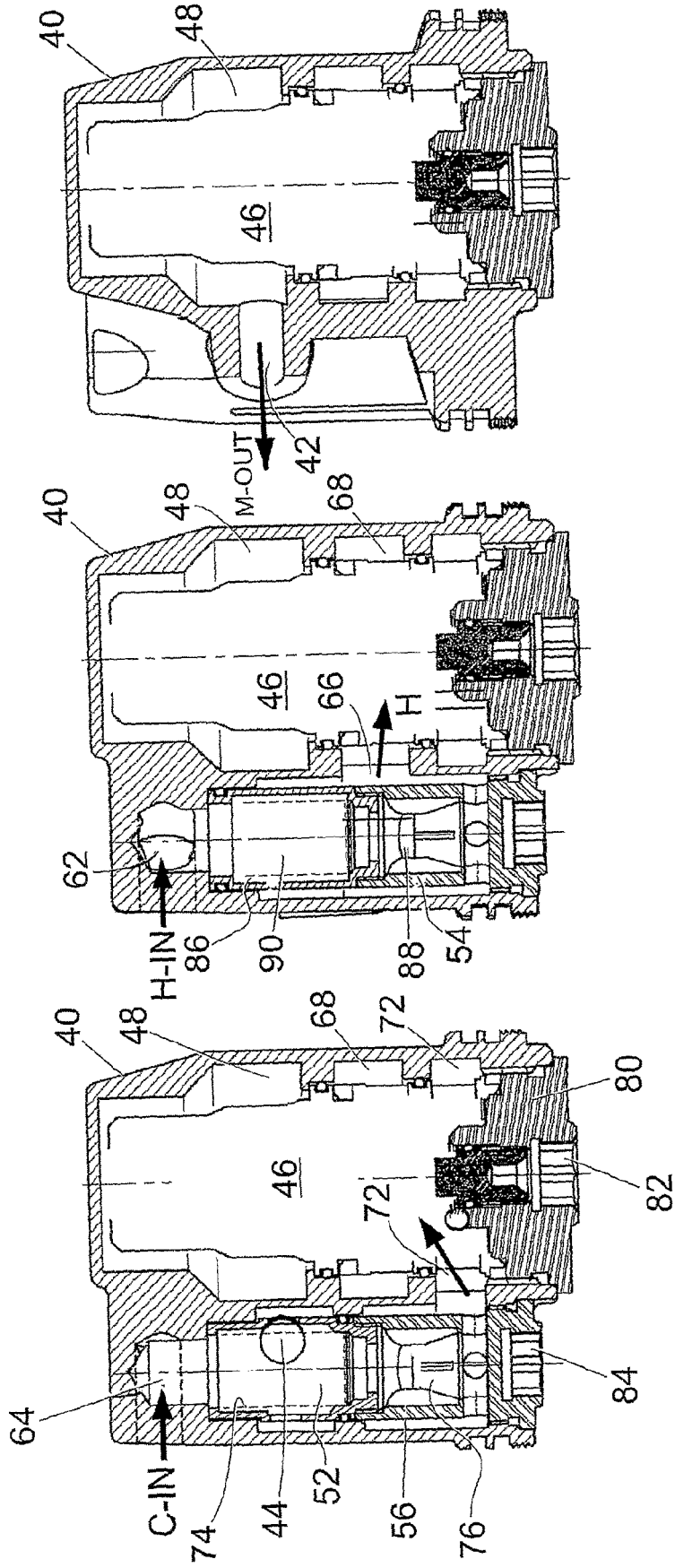
Fig. 12 (M-M)
