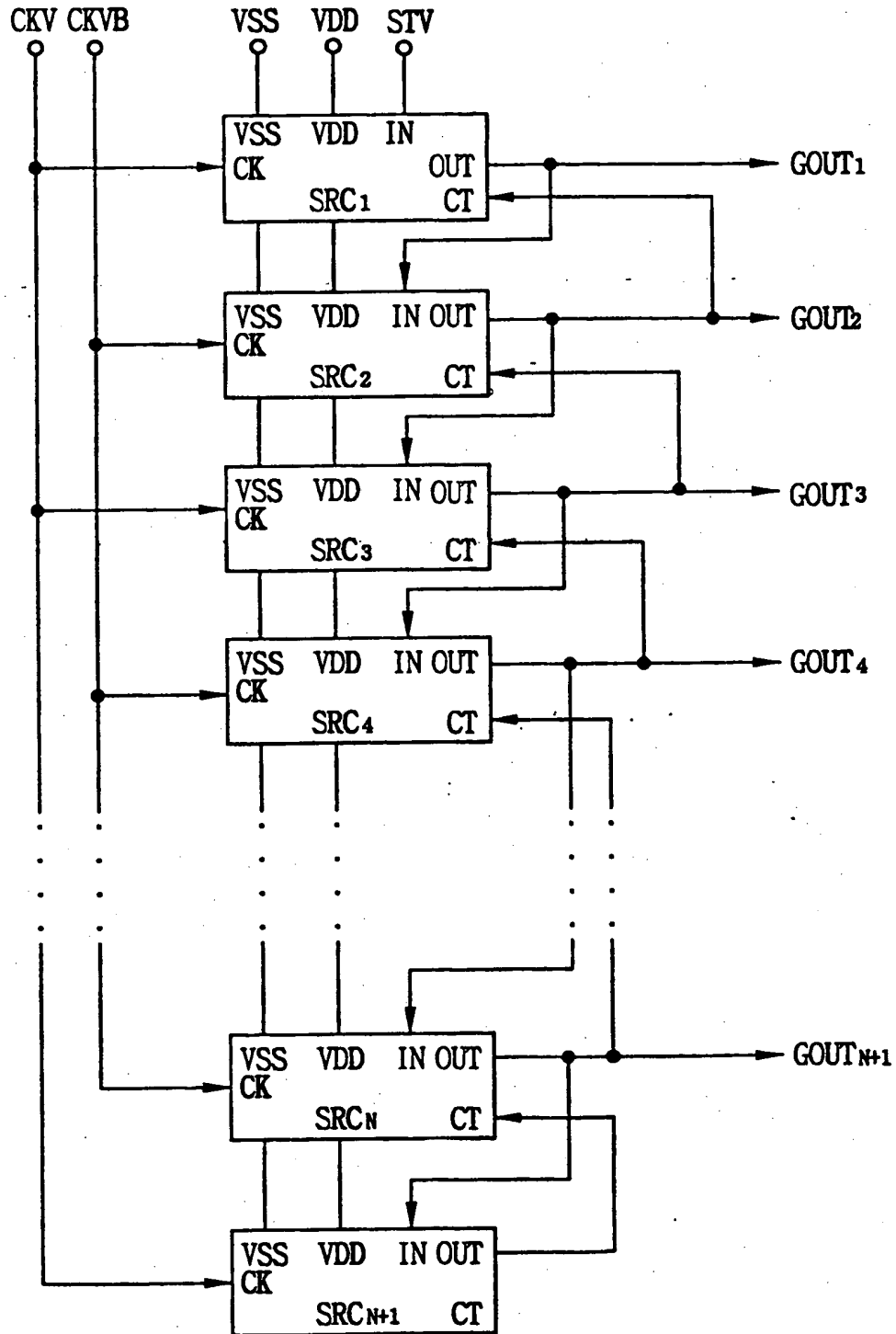
FIG.2 (PRIOR ART)
