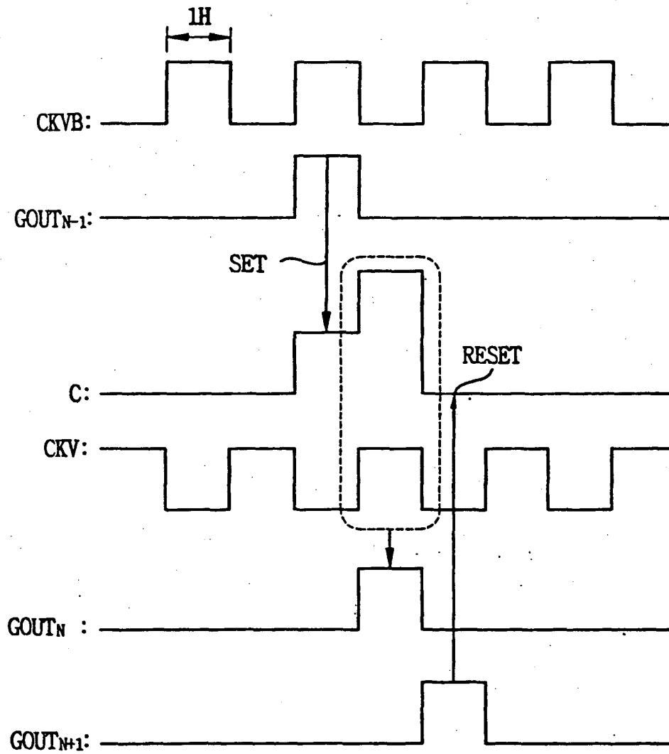
FIG. 3 (PRIOR ART)
