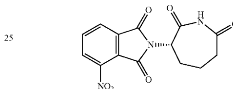
4-Nitro-2-[(3S)-2-oxoazepan-3-yl]isoindoline-1,3-dione (Compound 5)
