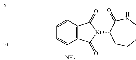
4-Amino-2-[(3S)-2-oxoazepan-3-yl]isoindoline-1,3-dione (Compound 8)
