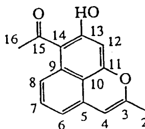
RM 18b (11)
