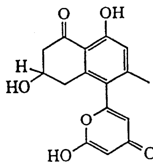
MUTACTIN (6)
