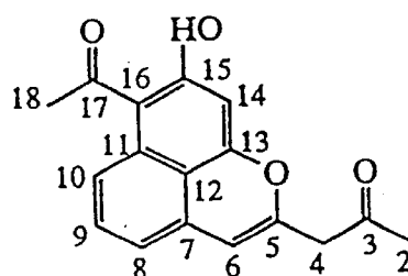
RM 18 (10)
