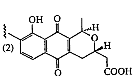
ACTINORHODIN (3)
