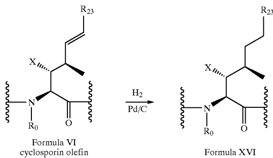
Scheme 17
