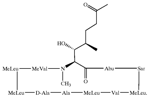
Formula XI
