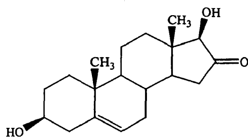
compound 8
