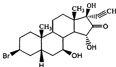
subgroup 12-2,
