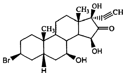
subgroup 12-1,
