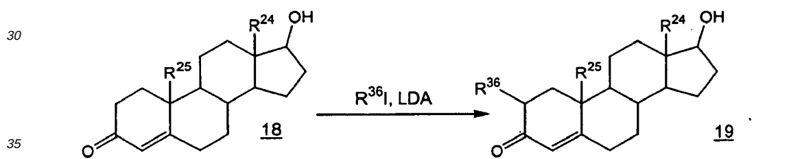
Scheme 13
