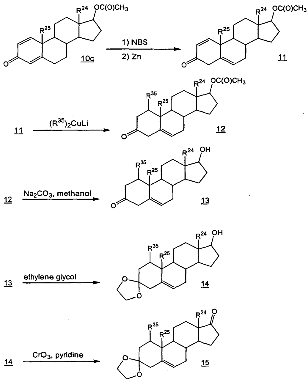
Scheme 11
