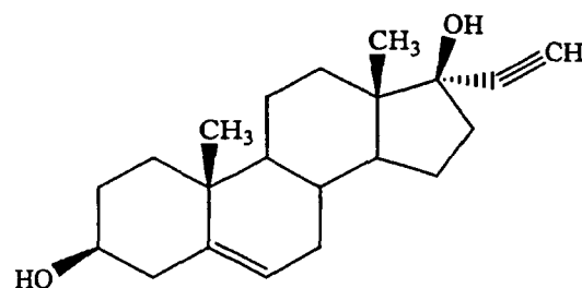
compound 6
