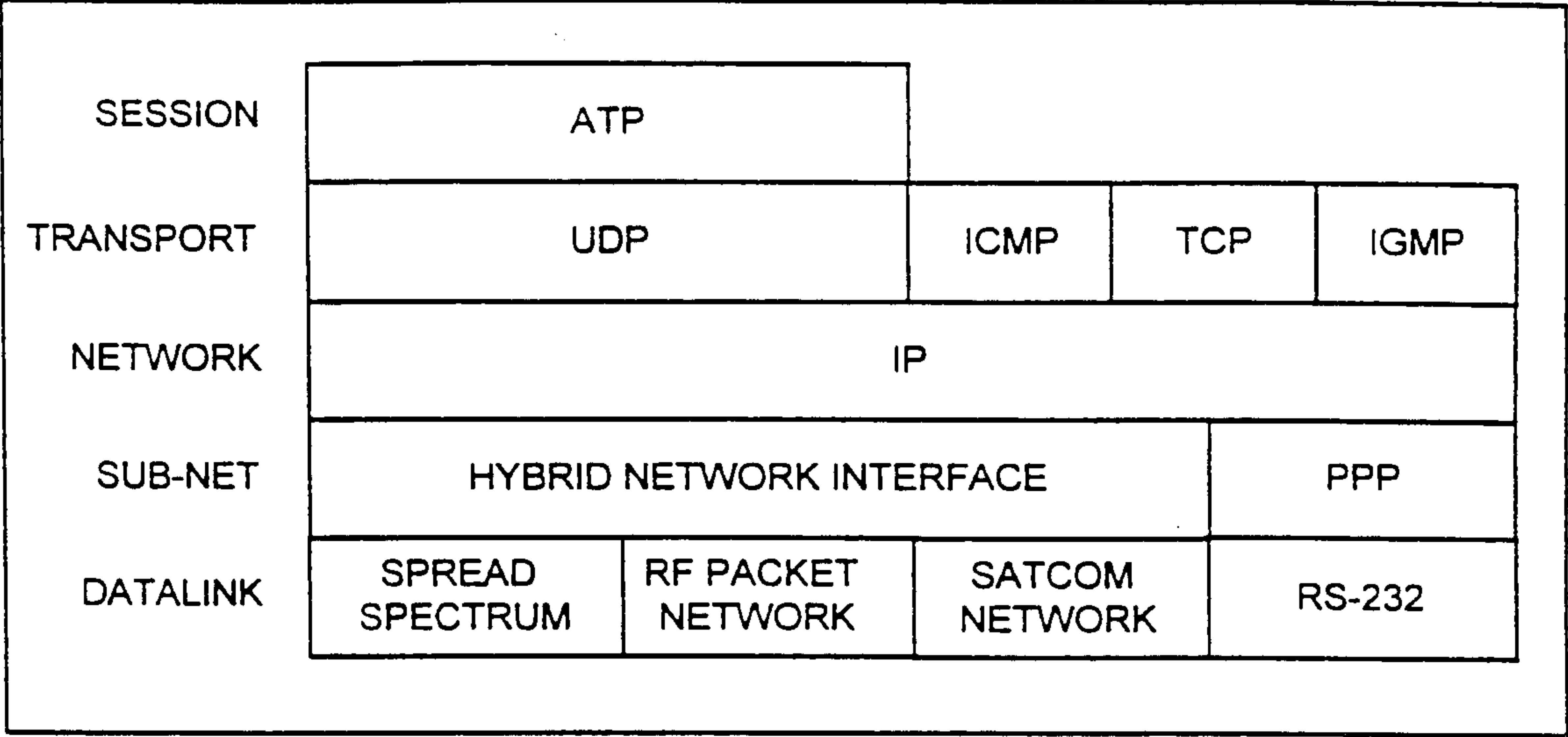
FIG. 9 Protocol Stack
