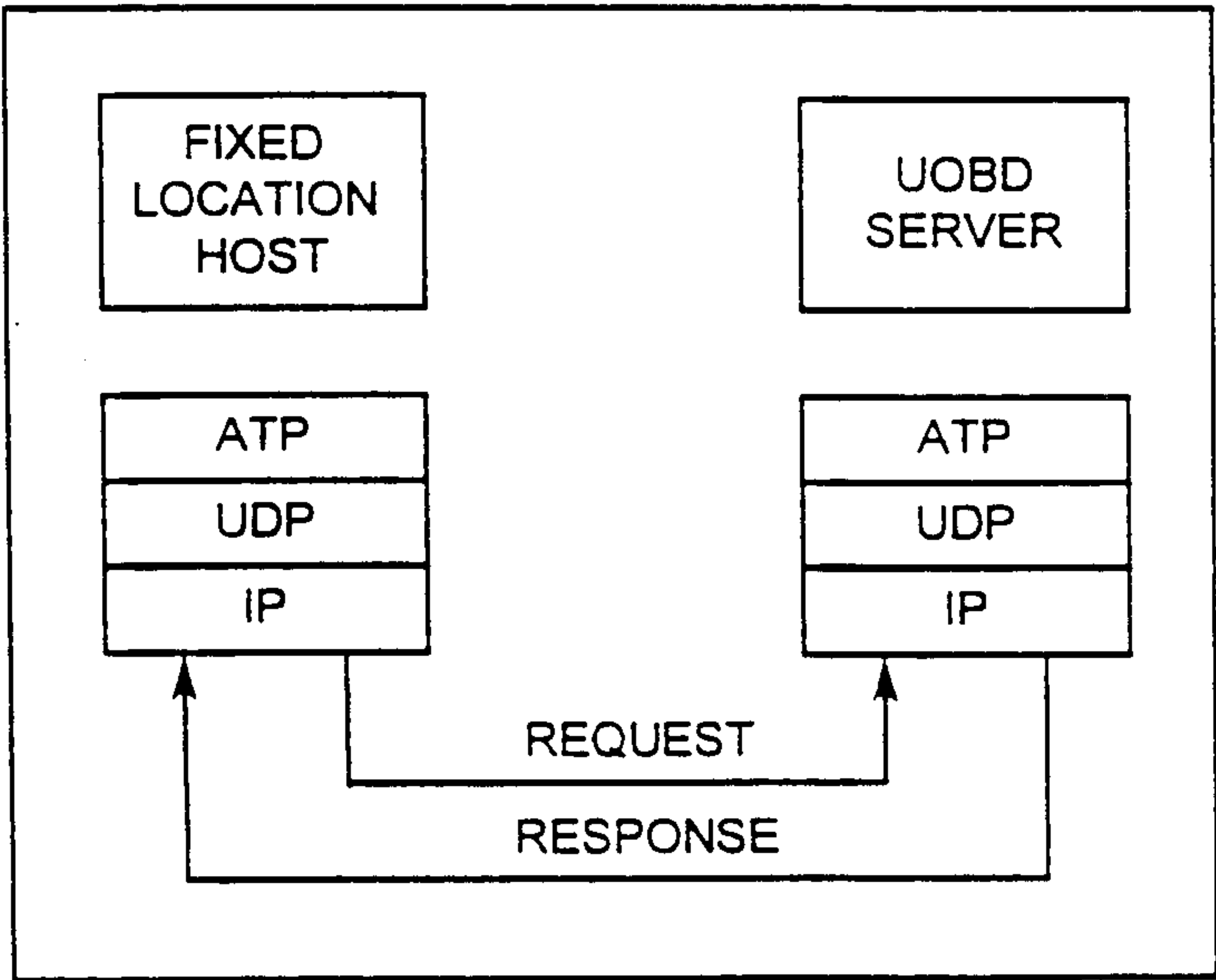
FIG. 10 Automotive Telemetry Protocol
