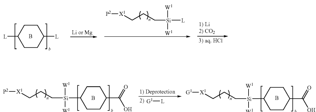
[Reaction Scheme 4]
