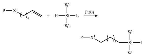
[Reaction Scheme 5]
