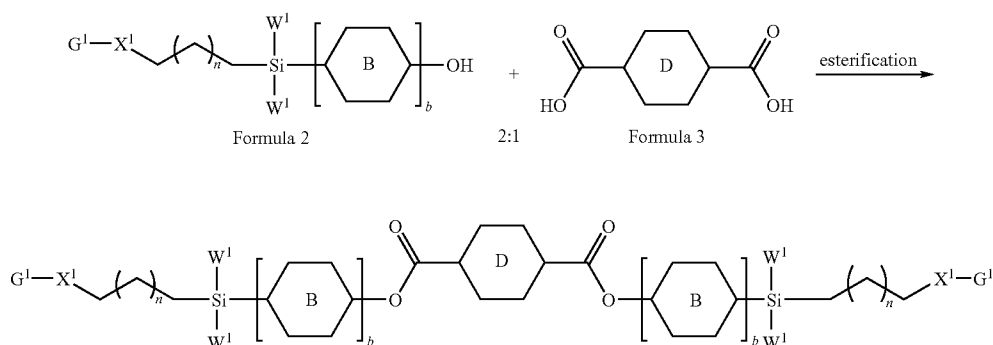
[Reaction Scheme 1]
