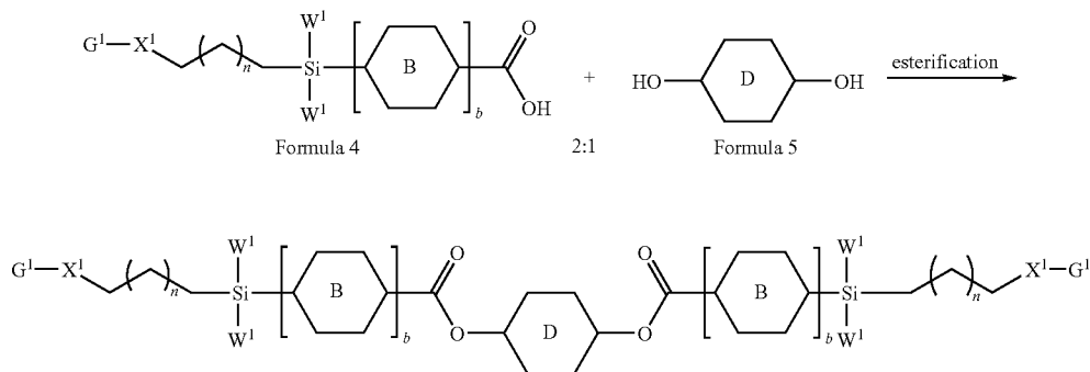
[Reaction Scheme 2]
