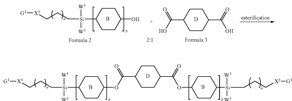
[Reaction Scheme 1]
