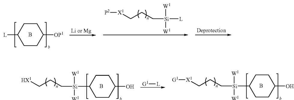
[Reaction Scheme 3]
