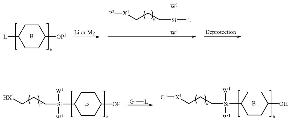
[Reaction Scheme 3]
