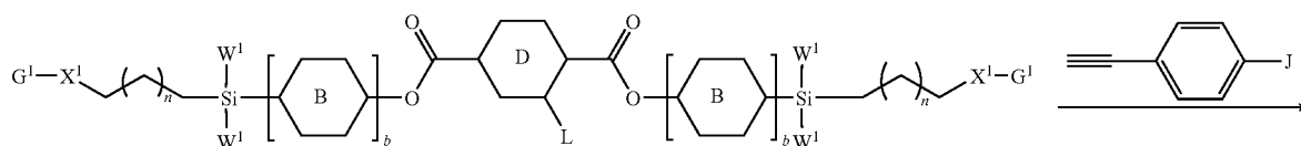
Formula 6
