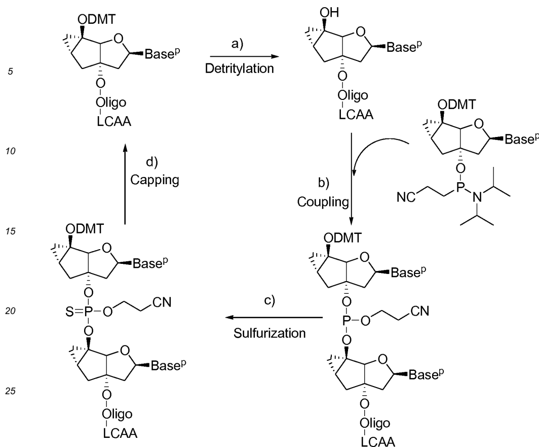
Scheme 1: General protocol for the synthesis of tricyclo-phosphorothioate-DNA (tc-DNA-PS)
