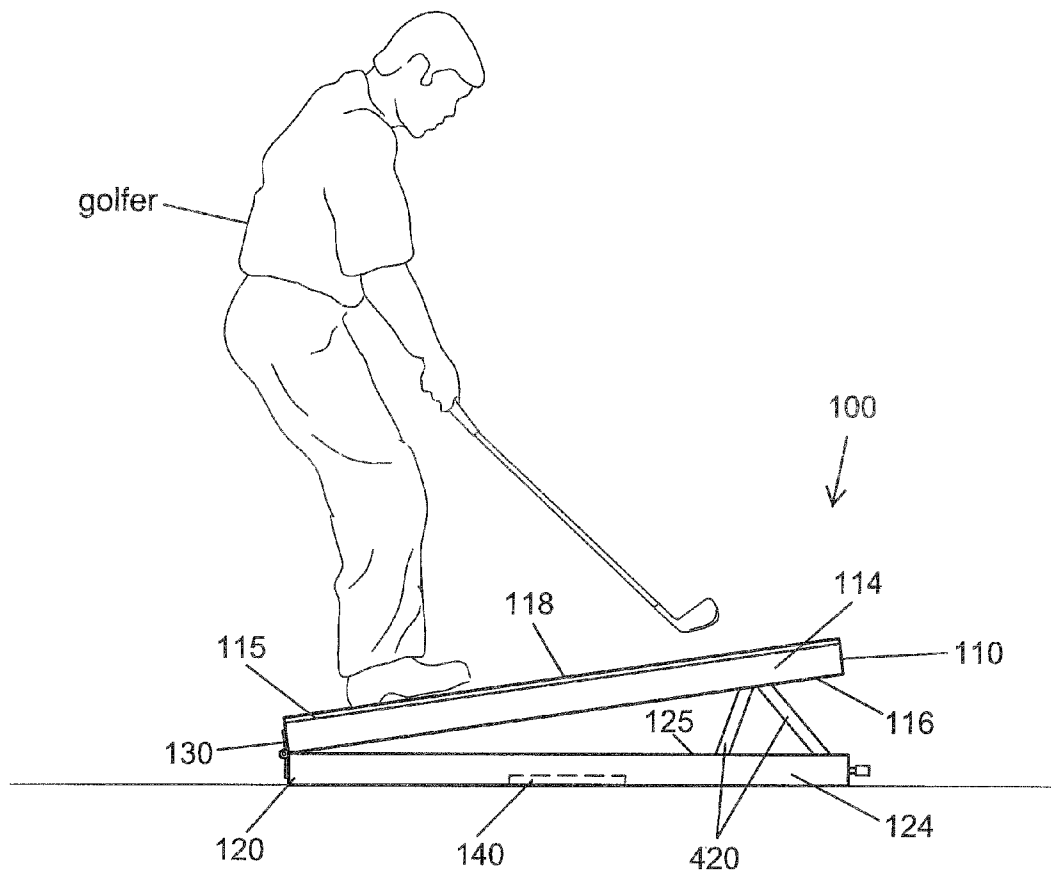
FIG. 6 (In-use View)
