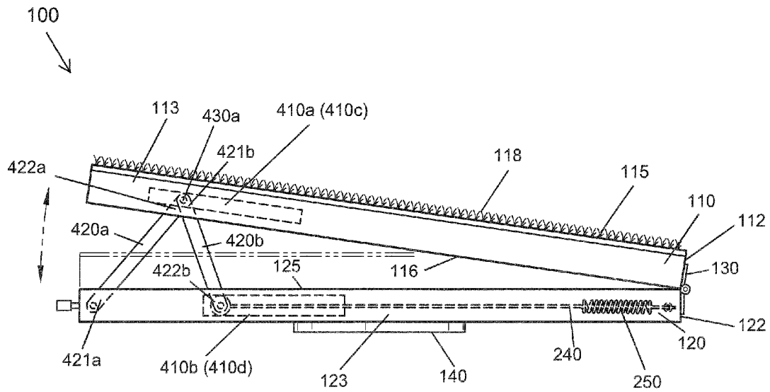
FIG. 3 (Side View)
