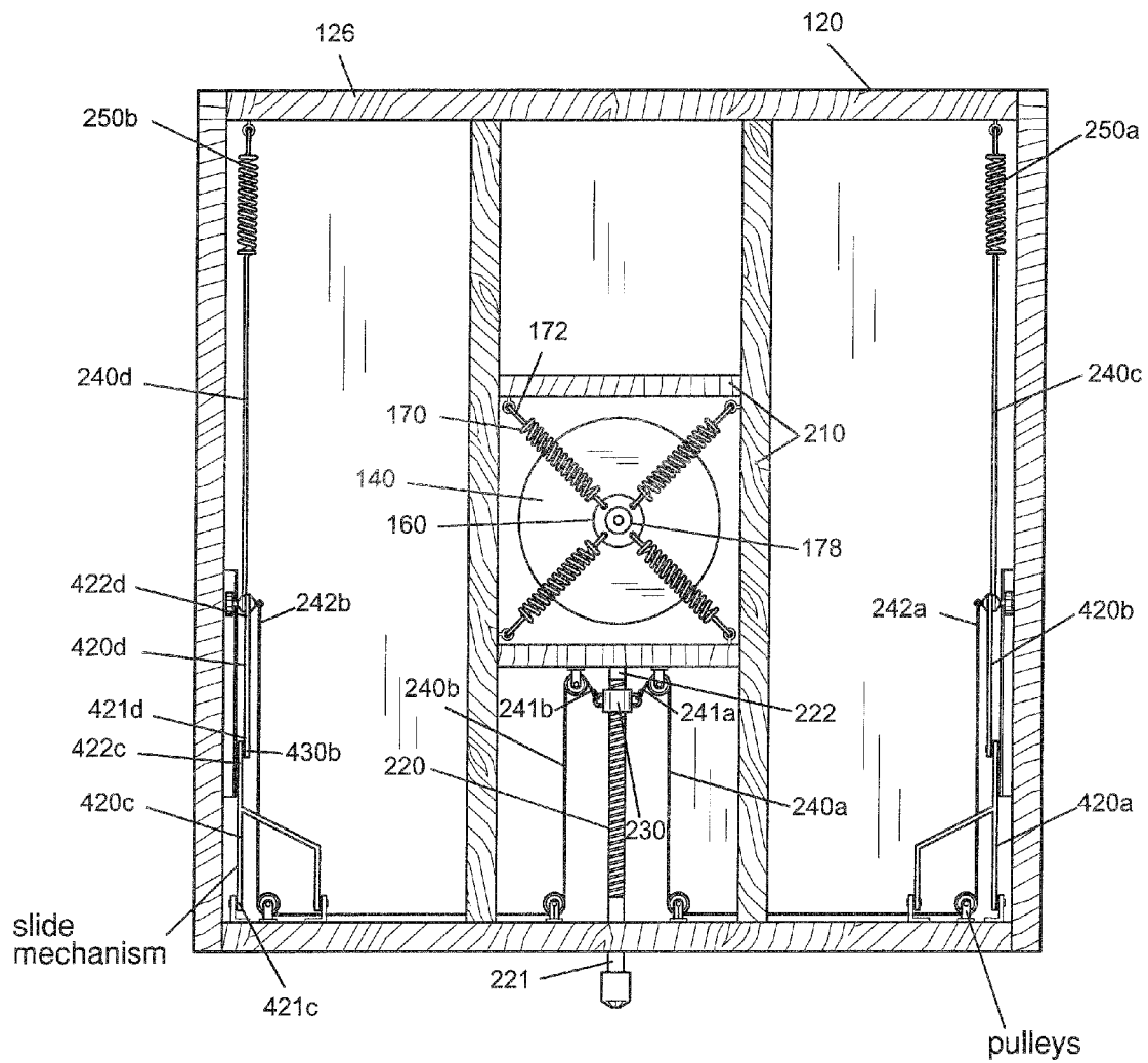
FIG. 5 (Cross-sectional View)
