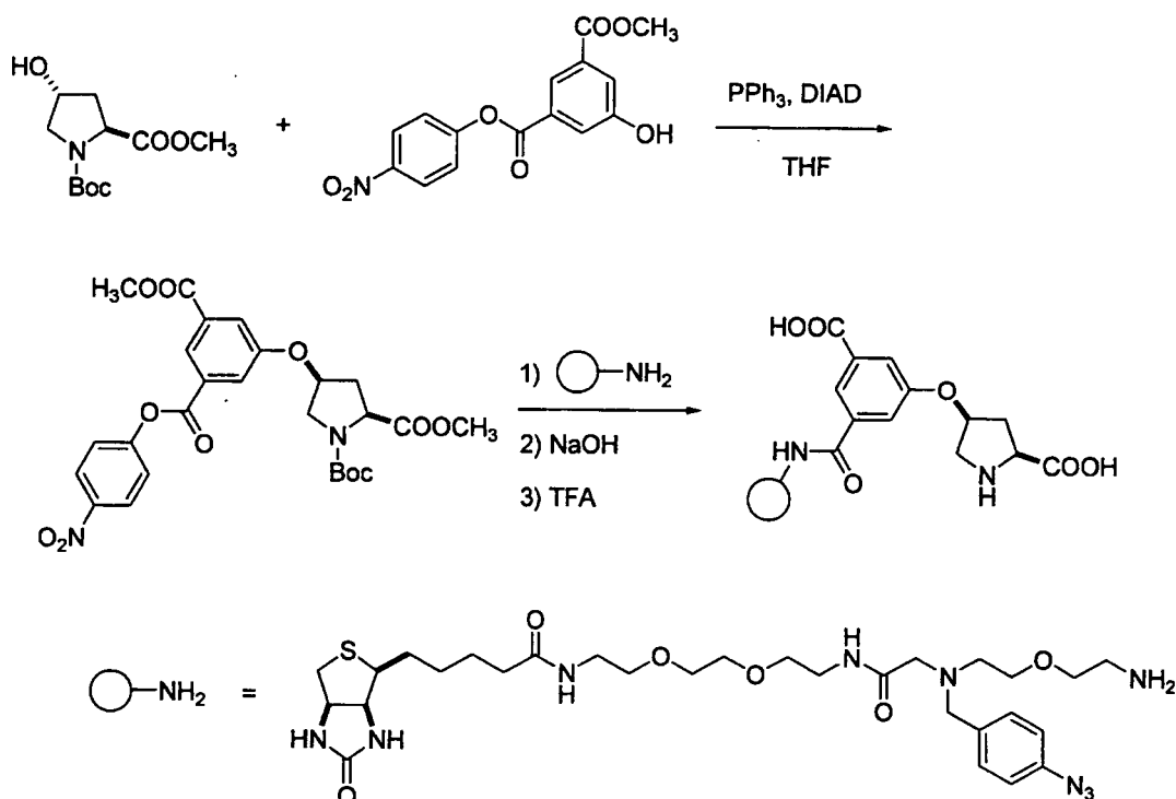
[Chemical Formula 66]
