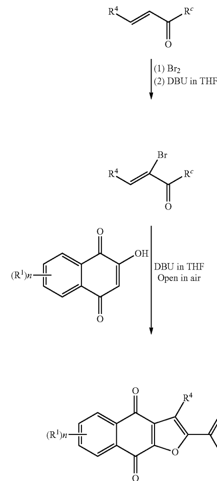
Scheme 1:
