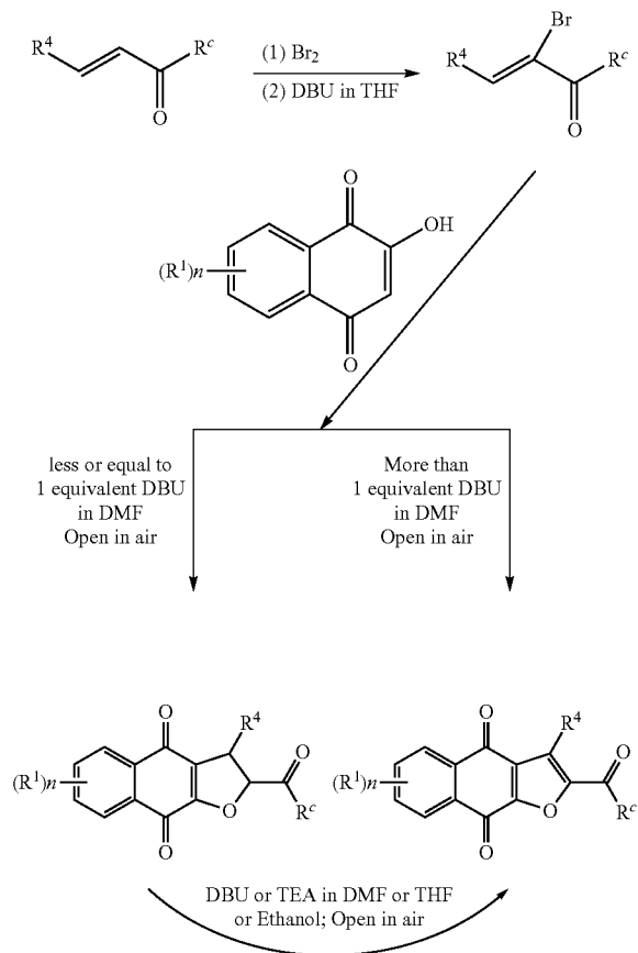
Scheme 2:
