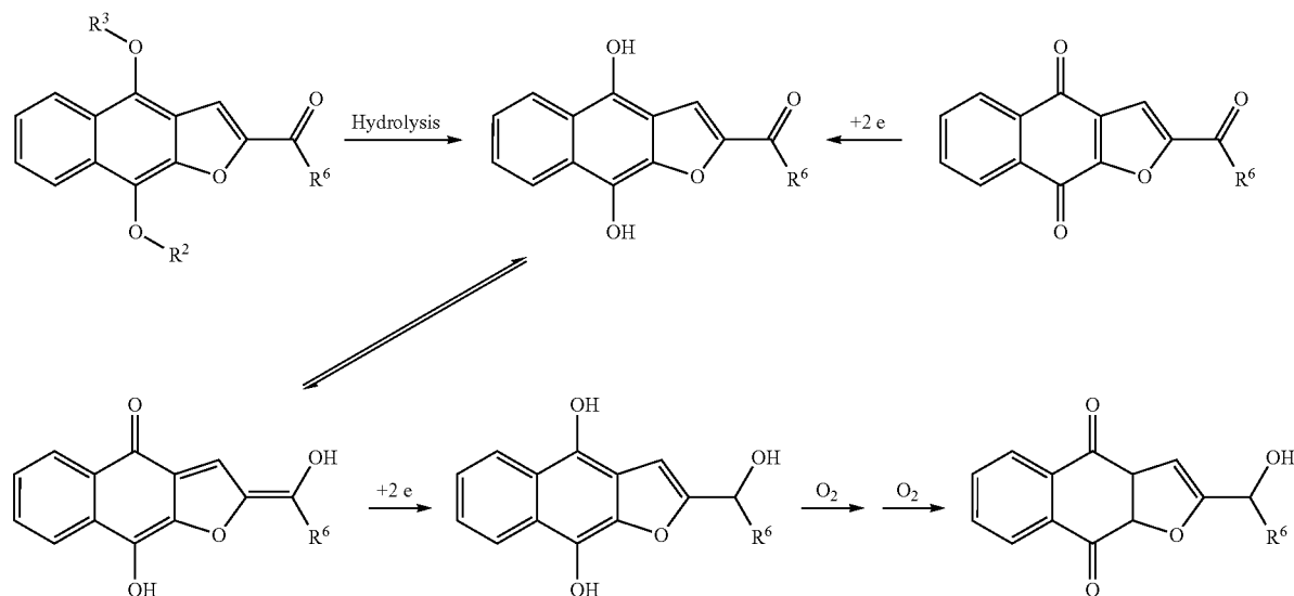
Scheme 7:
