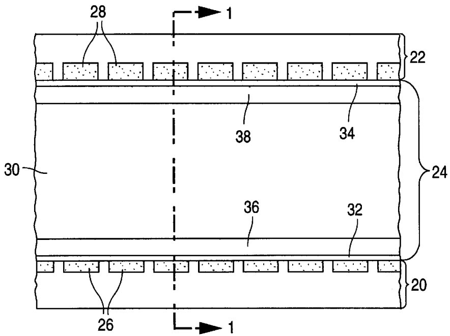
Fig. 2 PRIOR ART
