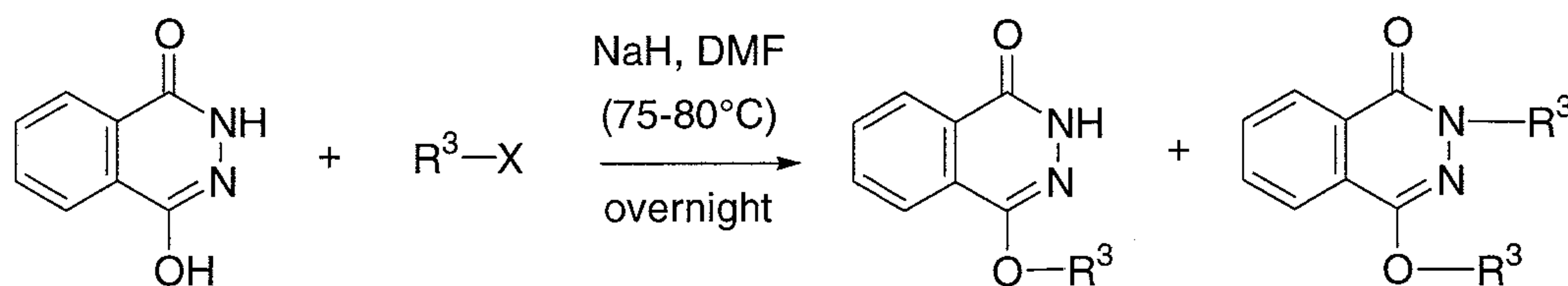
Scheme 1
