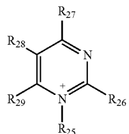
[Chemical Formula-29]
