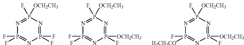
(cyclotriphosphazenes having ethyl group(s) through oxygen)
