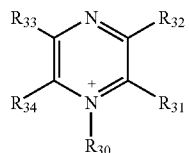
[Chemical Formula-30]
