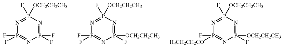
(cyclotriphosphazenes having propyl group(s) through oxygen)
