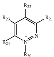
[Chemical Formula-27]
