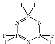
(cyclotriphosphazene wholly substituted with fluorine atoms)
