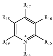
[Chemical Formula-27]
