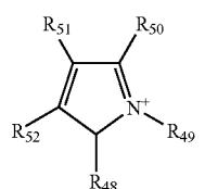
[Chemical Formula-34]
