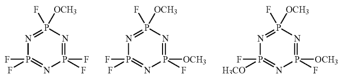
(cyclotriphosphazenes having methyl group(s) through oxygen)
