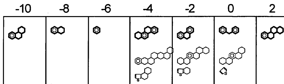
Figure 9 1-Ring Aromatic Cores
