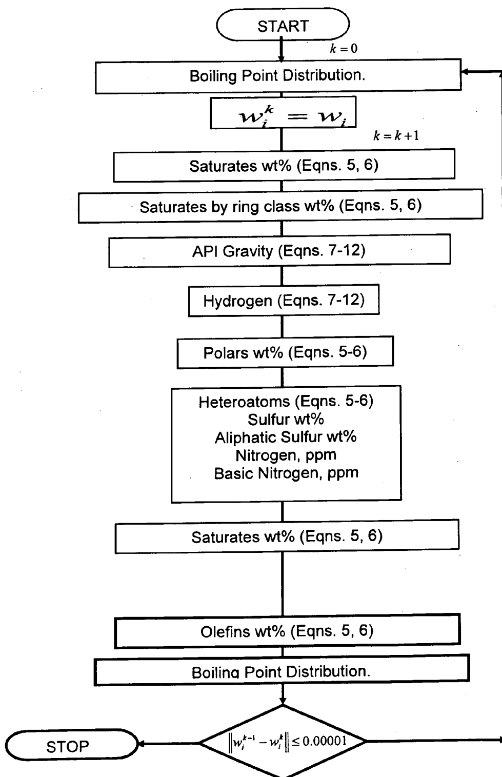
Figure 17 Iterative Model-of-Composition Synthesis Algorithm
