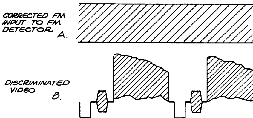
FIG.18 FM DISCRIMINATOR
