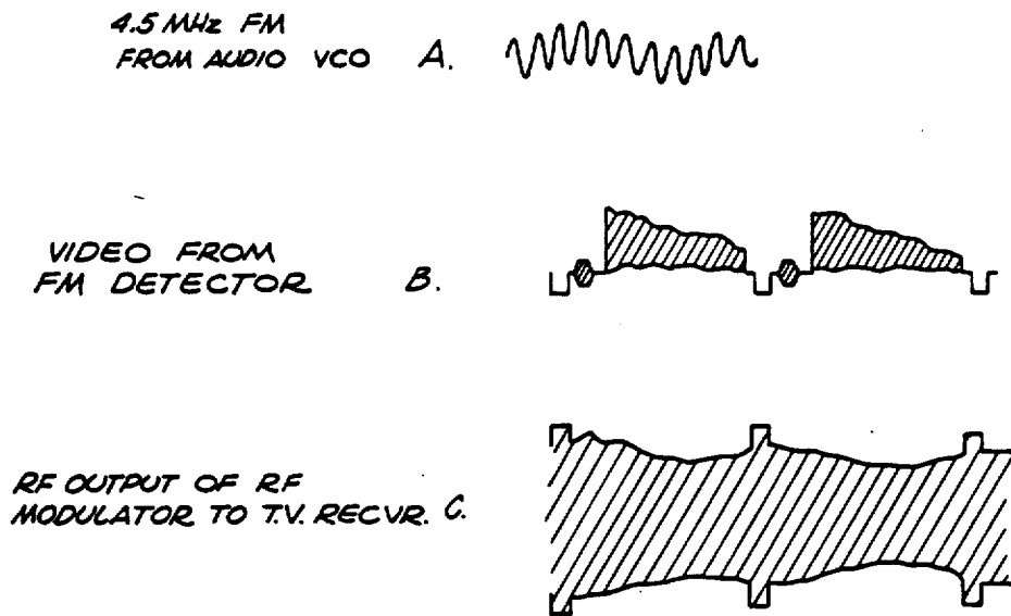
FIG. 25 RF MODULATOR
