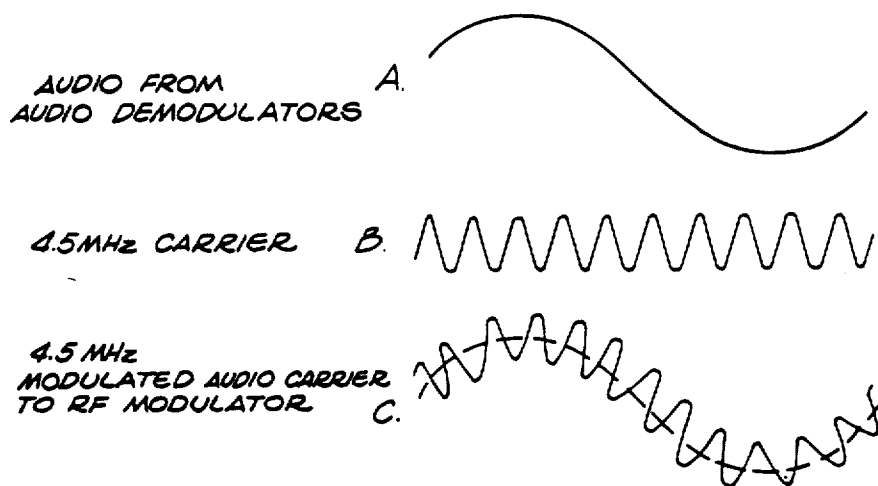
FIG. 23 4.5 MHz VCO AUDIO MODULATOR
