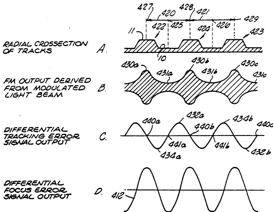
FIG. 8 SIGNAL RECOVERY
