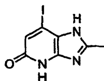
7-iodo-2-methyl-1,4-dihydro-imidazo[4,5-b]pyridin-5-one
