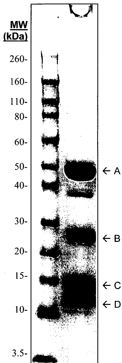
Figure 1: SDS-PAGE
