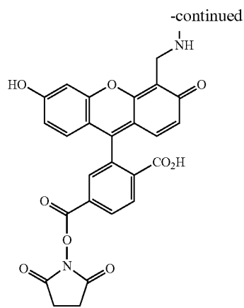
6-CFB-DTMR-2-NHS
