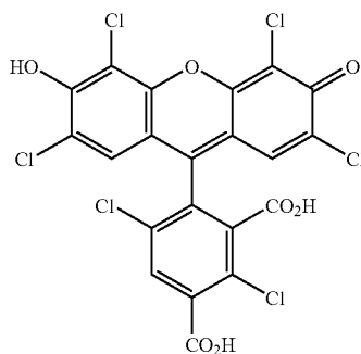
5-carboxy-HEX
