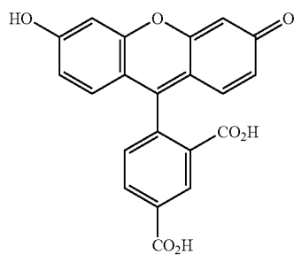
5-carboxyfluorescein
