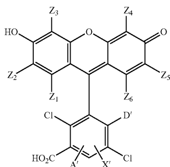
4,7-Dichlorofluorescein (See Pat. No. 5,188,934)
