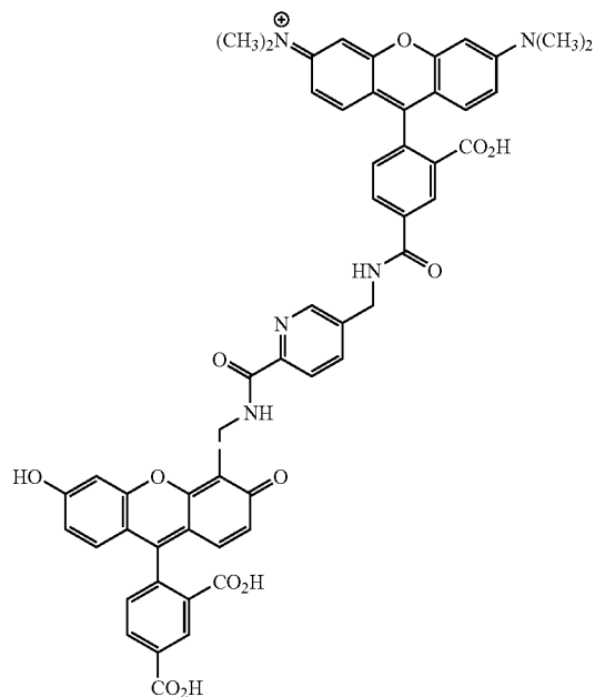
5-TMR-P-CF
