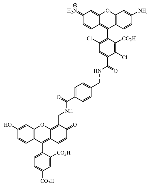
5-CFB-DR110-2
