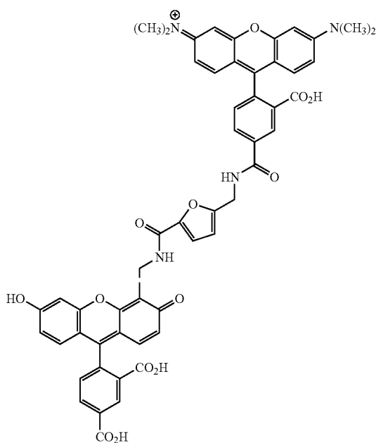
5-TMR-F-CF
