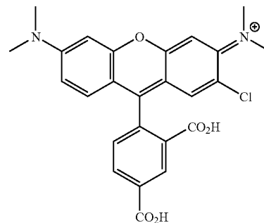
5-carboxyrhodamine
