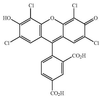
ZOE
