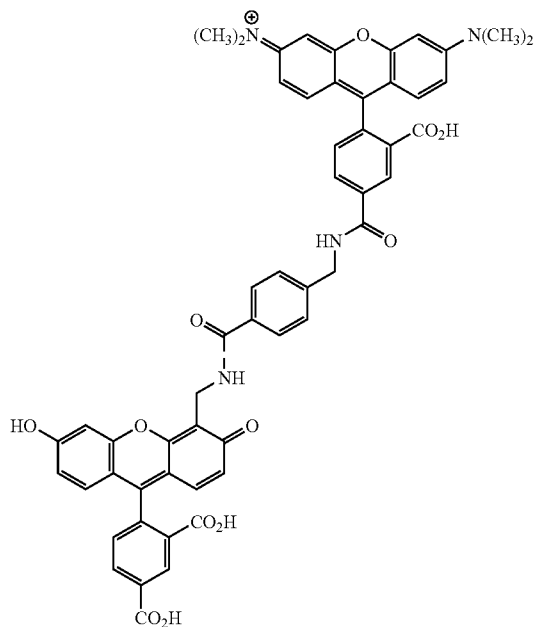
5-TMR-B-CF
