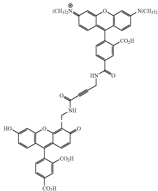
5-TMR-A-CF
