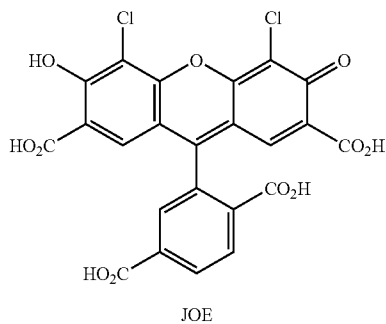
JOE
