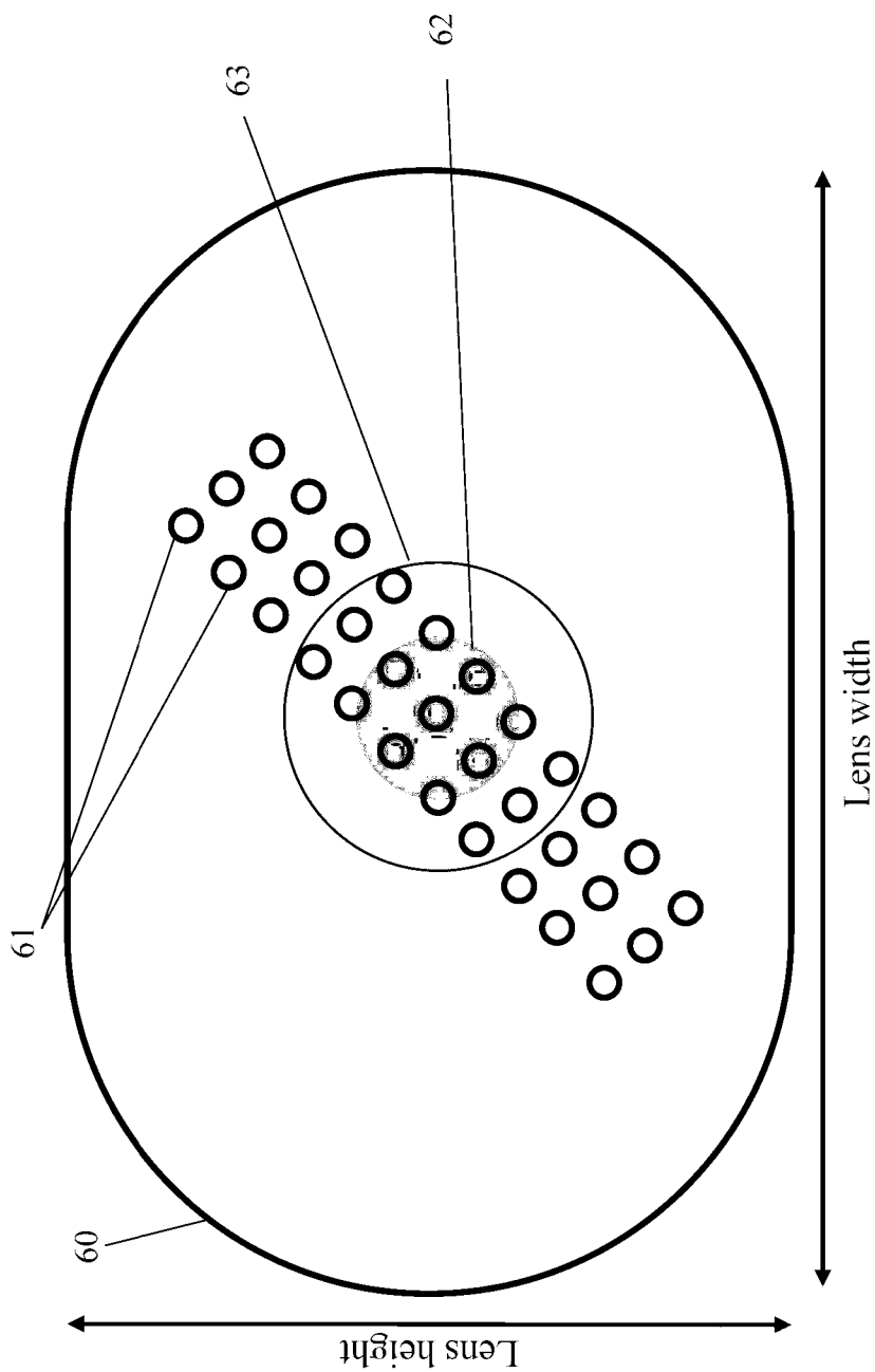
Refractive optical elements (ROE) embedded into a spectacle lens FIGURE 17C
