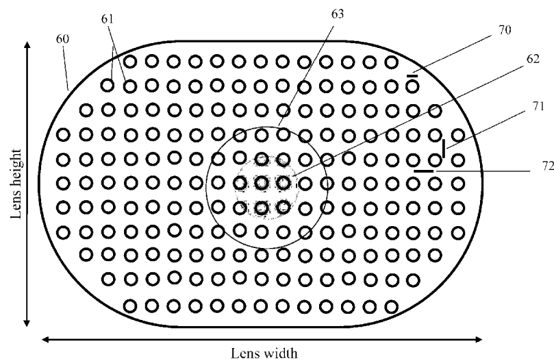
Refractive optical elements (ROE) embedded into a spectacle lens
