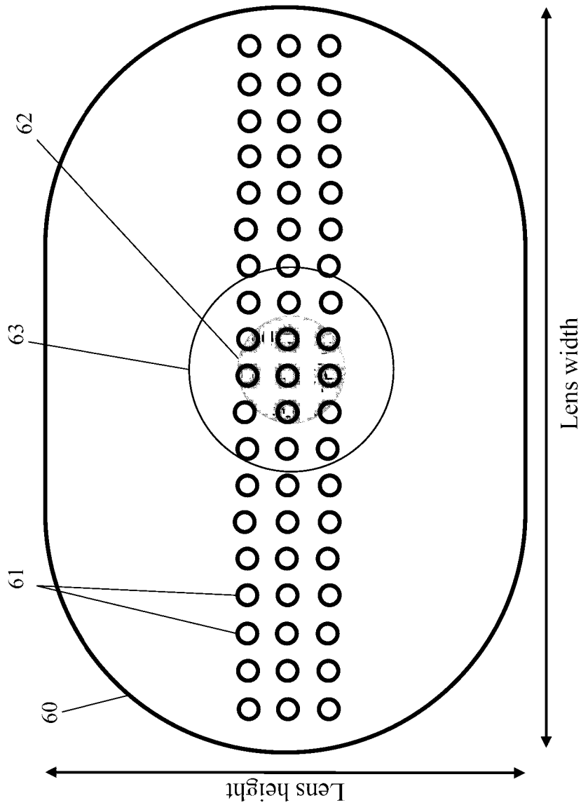
Refractive optical elements (ROE) embedded into a spectacle lens FIGURE 17A
