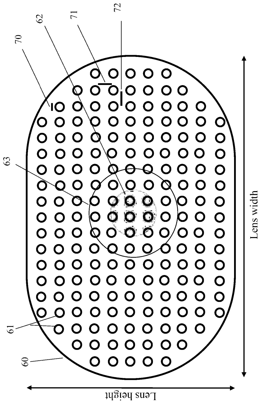
Refractive optical elements (ROE) embedded into a spectacle lens FIGURE 13A
