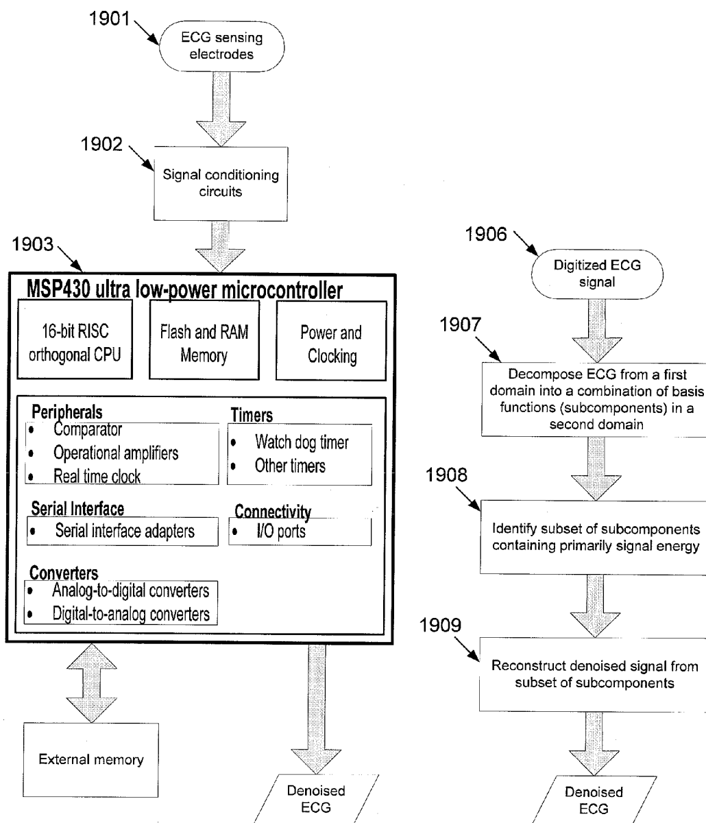
Figure 19 Apparatus for Improving SNR
