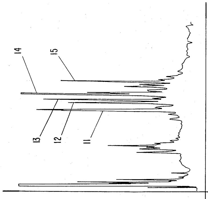
GLC PROFILE FOR EXAMPLE IV
