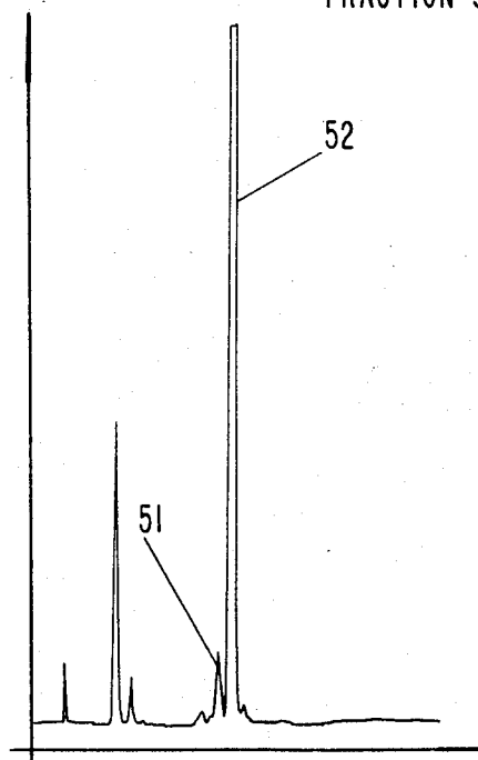
FIG. 19 GLC PROFILE FOR EXAMPLE V-A FRACTION 3
