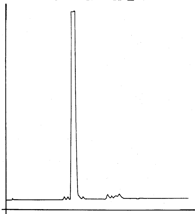
FIG. 17 GLC PROFILE FOR EXAMPLE V-A
