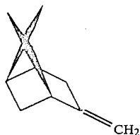
FIG. 18 is the GLC profile for the reaction product of Example V(A) containing the compound defined according to the structure:
