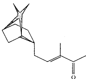
FIG. 10 is the NMR spectrum for the peak indicated by reference numeral "15" of the GLC profile of FIG. 8 containing a component of the reaction product of Example IV having the structure:
