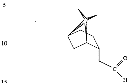
FIG. 22 is the GLC profile for fraction 6 of the reaction product of Example V(B) (conditions: 10' × 1/8" 5% Carbowax column programmed at 100°-220° C. at 4° C. per minute) containing the compound having the structure:
