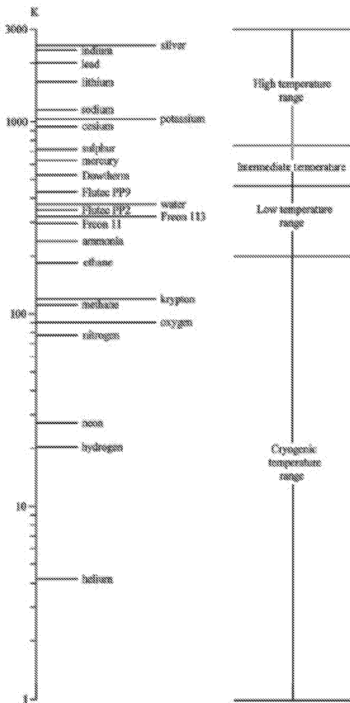
Operating temperature ranges of various working fluids
