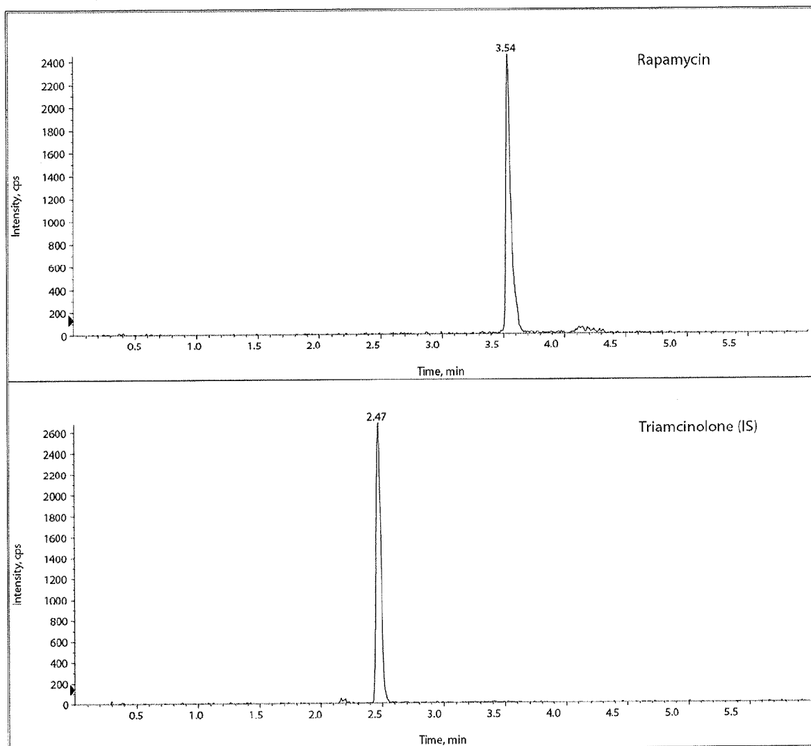
Representative Chromatograms of Rapamycin (top) and Internal Standard (bottom) in Lung Homogenate from Mouse 2-07 Administered Rapamycin by OPA Administration
