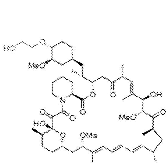
Everolimus (Affinitor)
