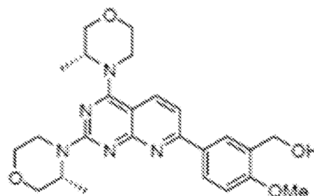
AZD8055
