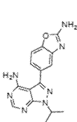
INK128
