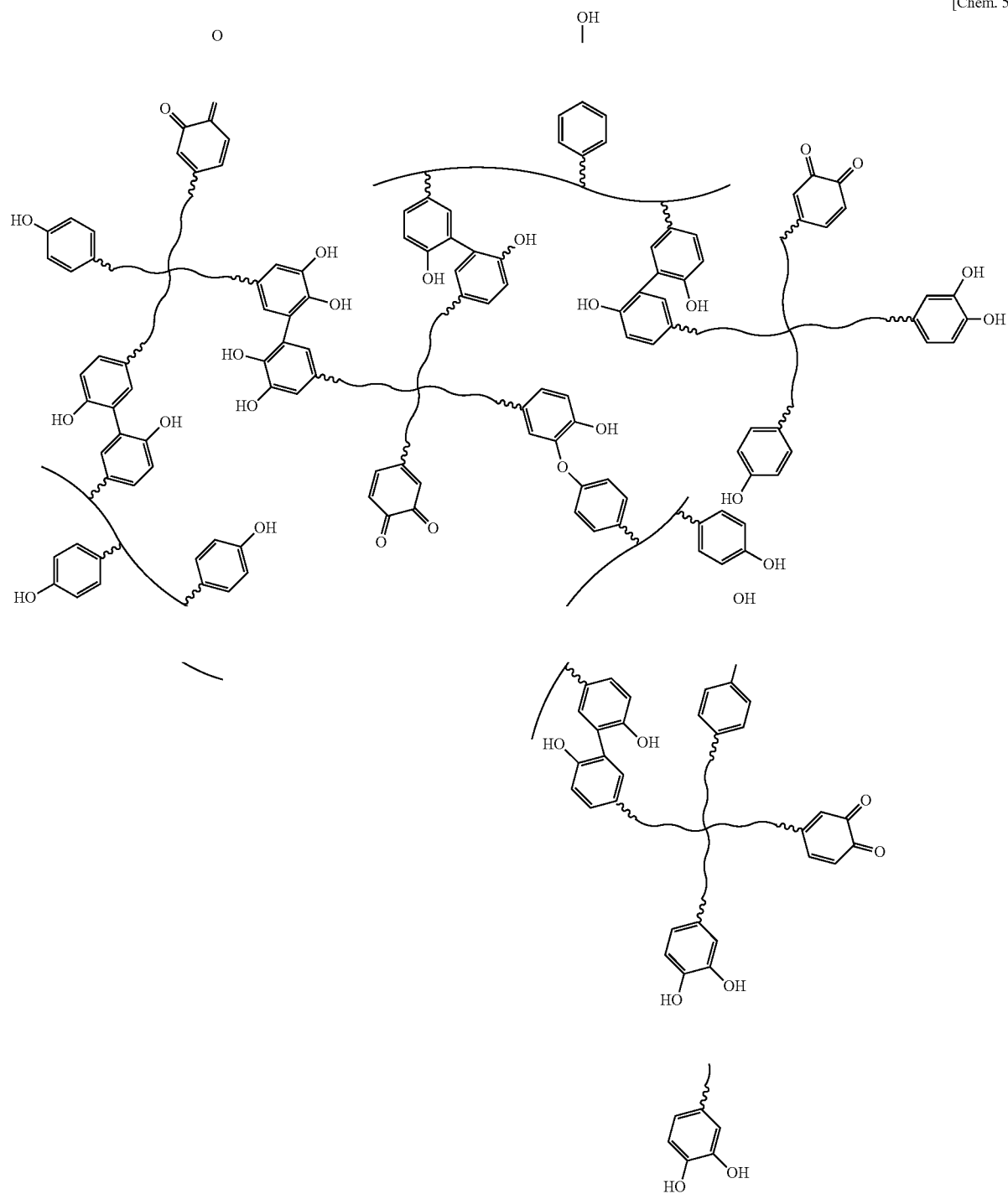
Chemistry Figure 5
