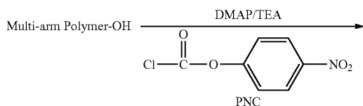
[Reaction Scheme 2]
