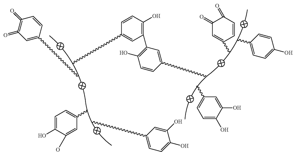
Chemistry Figure 7
