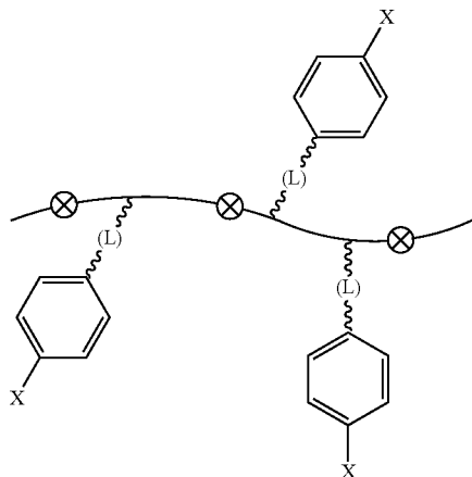
Chemistry Figure 2
