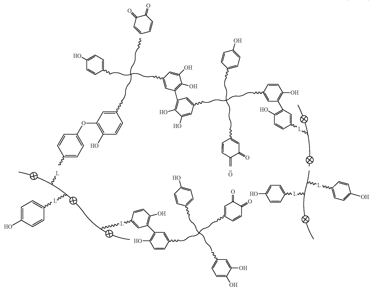
Chemistry Figure 7
