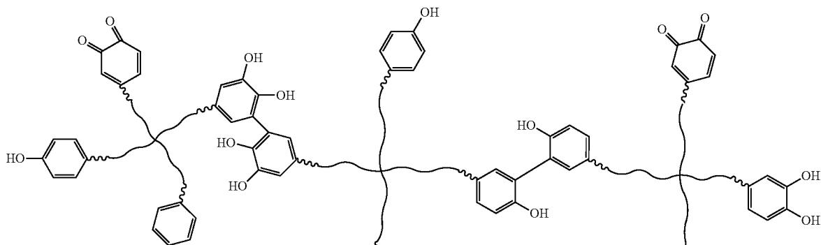
[Chemistry Figure 4]
