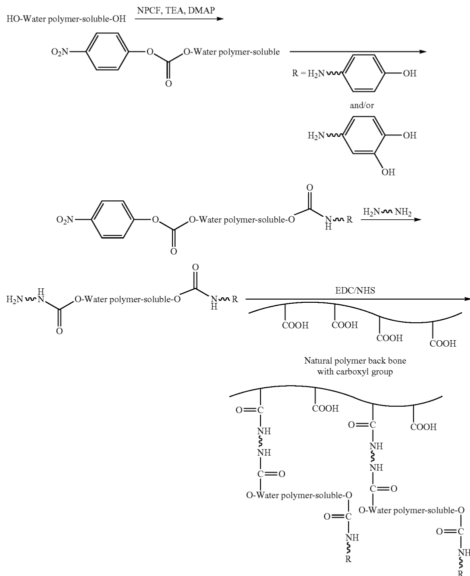
[Reaction Scheme 12]
