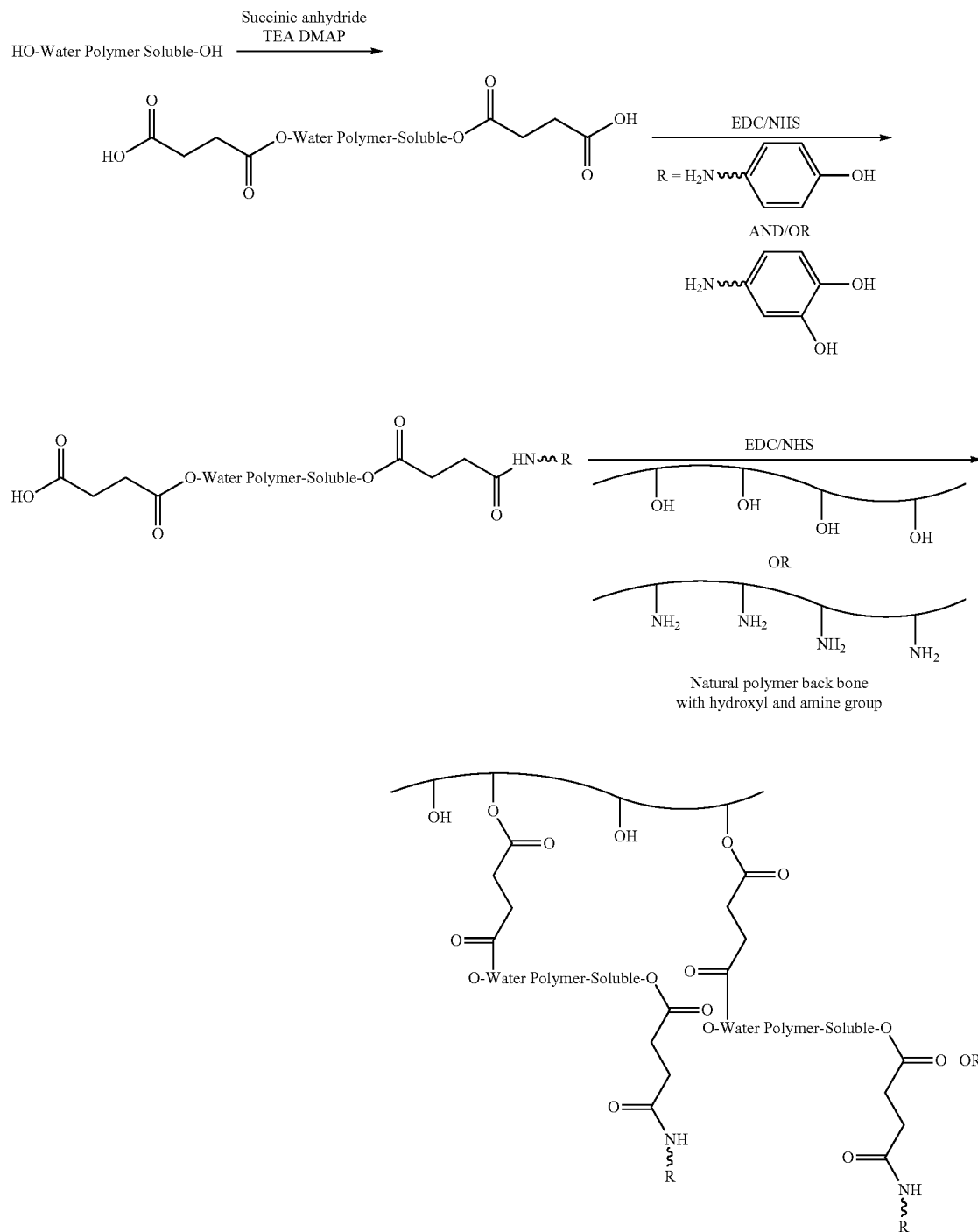
[Reaction Scheme 9]
