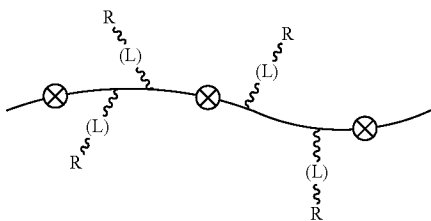
Chemistry Figure 3
