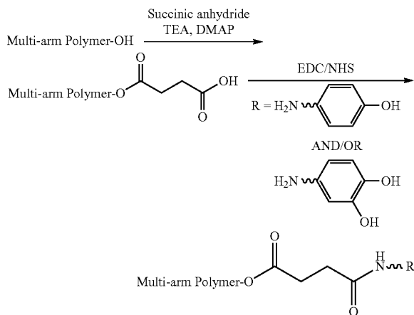
[Reaction Scheme 1]
