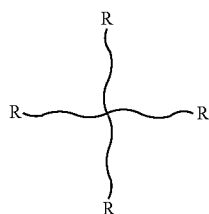
Chemistry Figure 2
