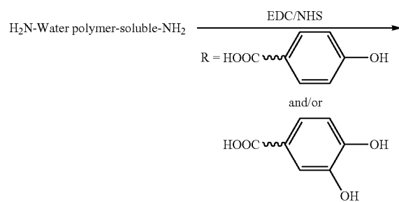
[Reaction Scheme 13]
