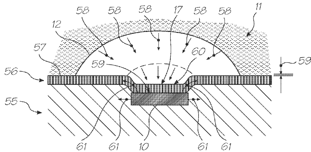
FIG. 57 (PRIOR ART)
