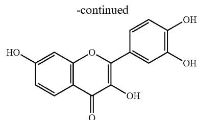
[3,3',4',7-Tetrahydroxyflavone]
