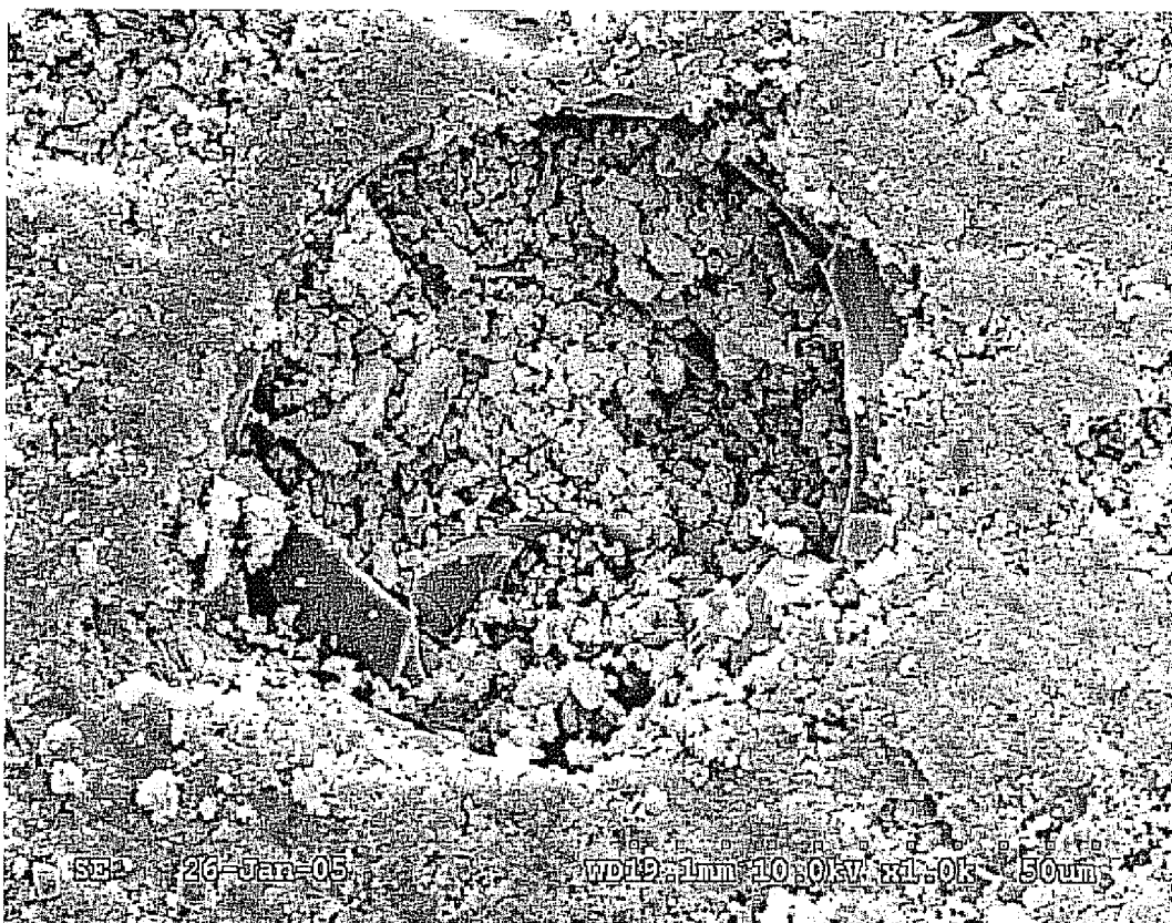
Figure 1. Sanded 85 micron hollow glass micro-sphere
