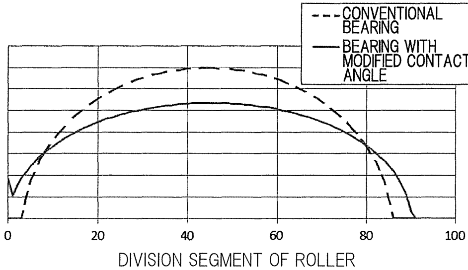
CONTACT SURFACE PRESSURE DISTRIBUTION ON REAR SIDE
