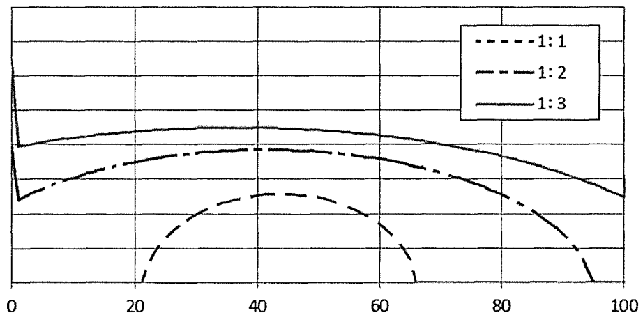
CONTACT SURFACE PRESSURE DISTRIBUTION ON FRONT SIDE
