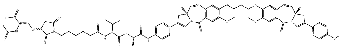
Compound 4
