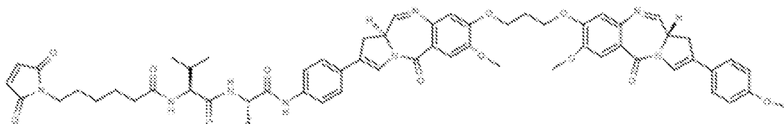
Compound 1
