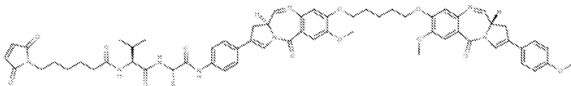
Compound 1
