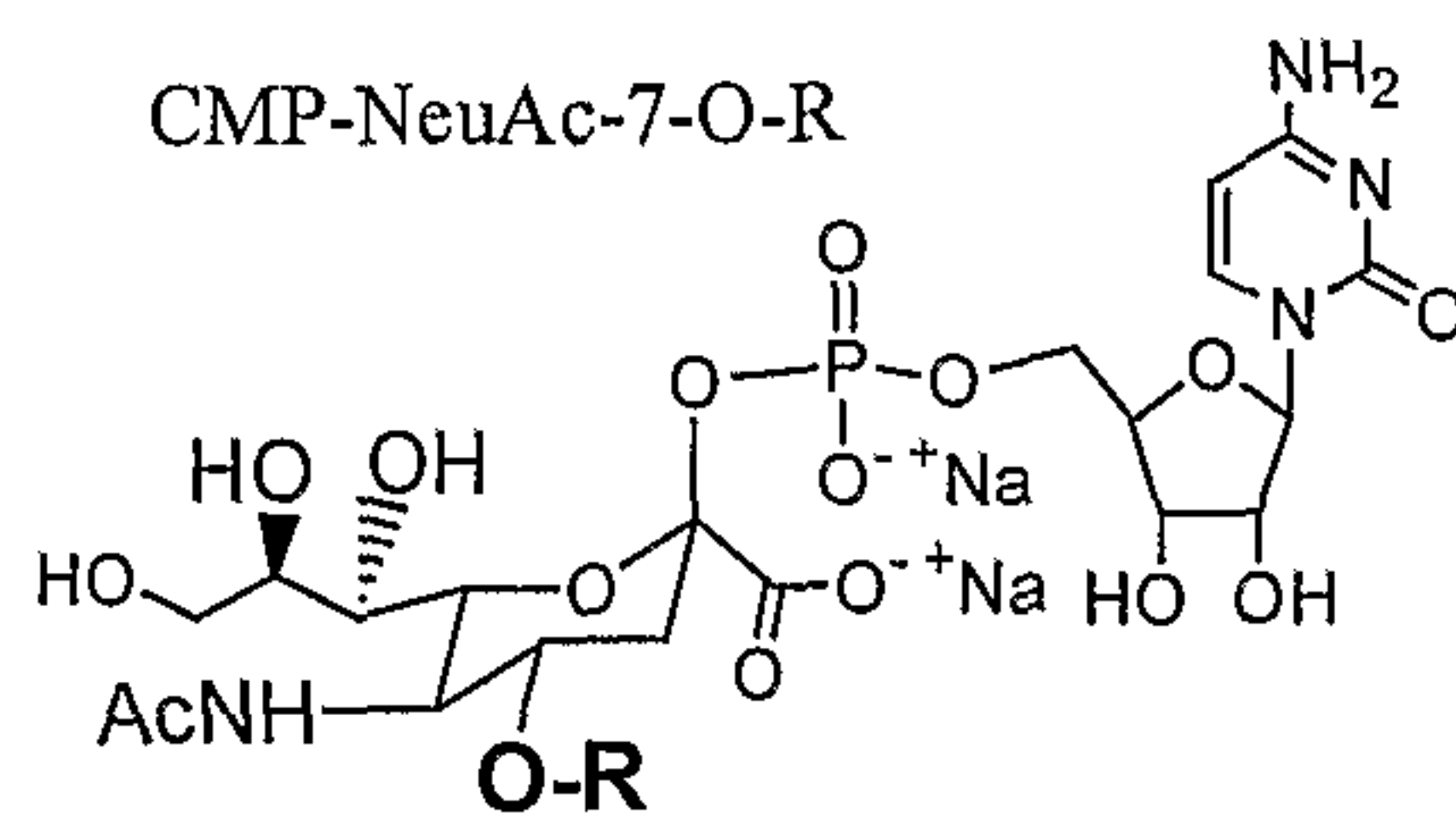
CMP-NeuAc-4-O-R
