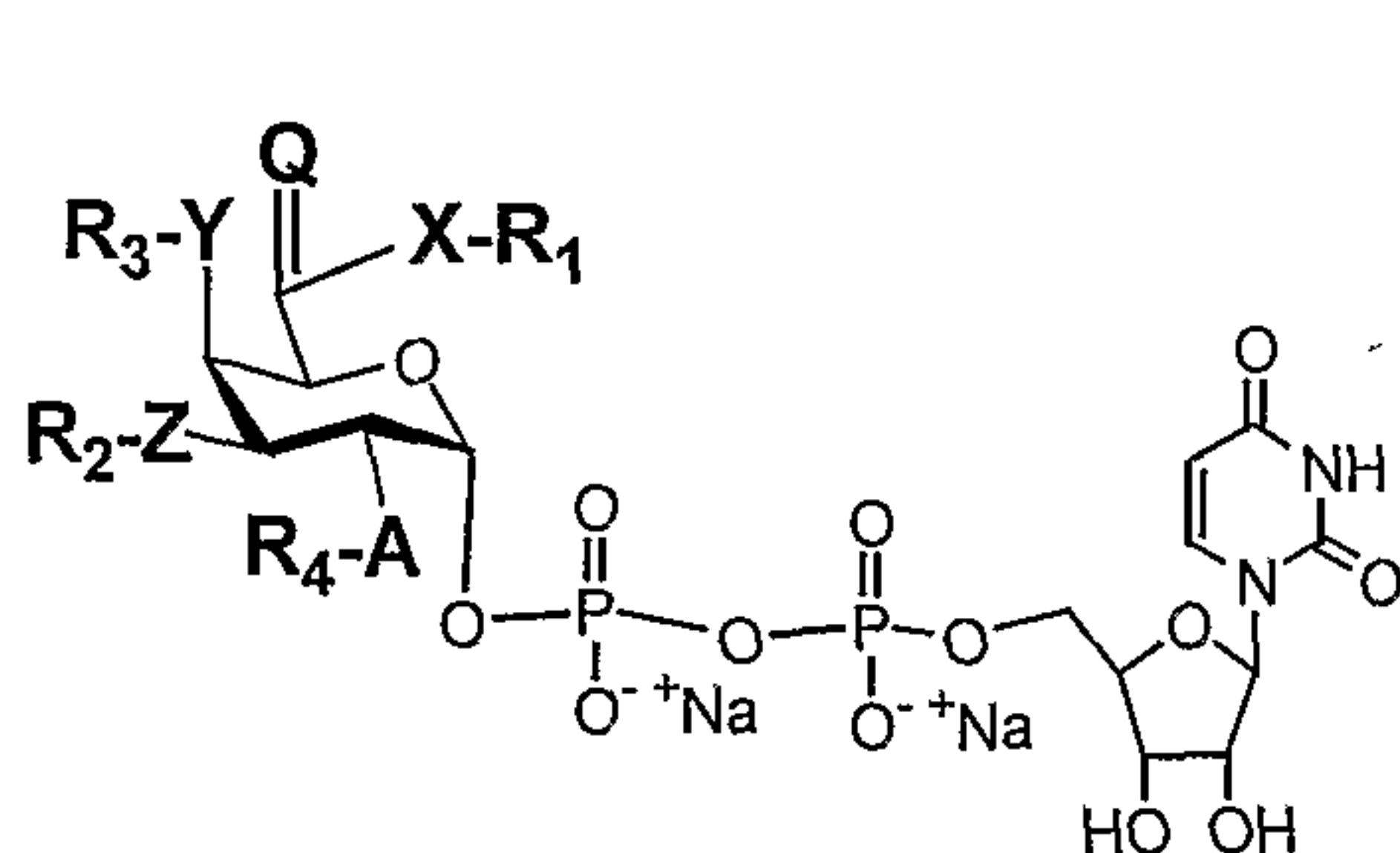
UDP-galactose-derivatives
