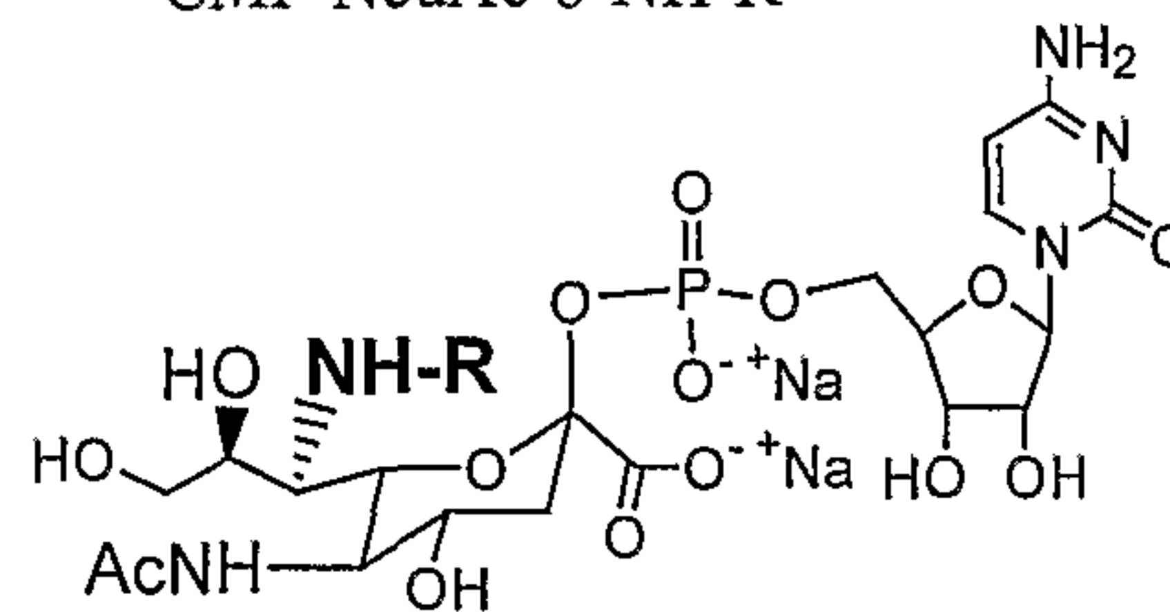
CMP-NeuAc-8-NH-R
