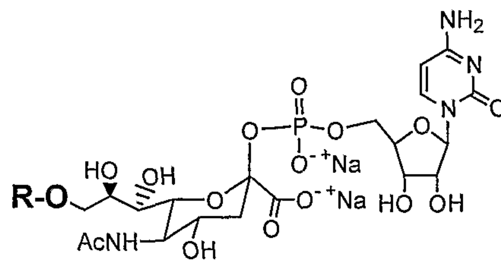
CMP-NeuAc-9-O-R
