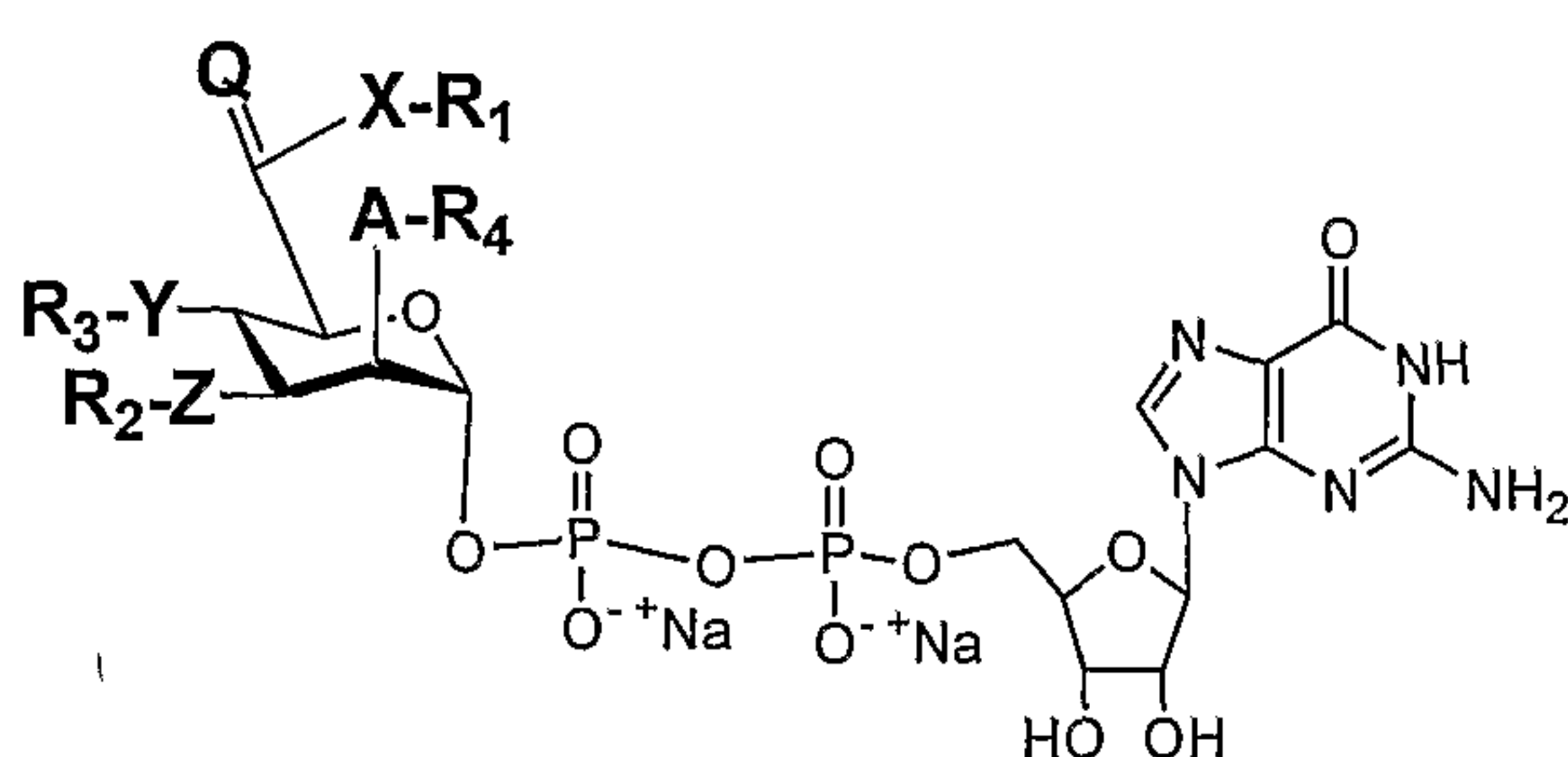
GDP-Mannose-derivatives
