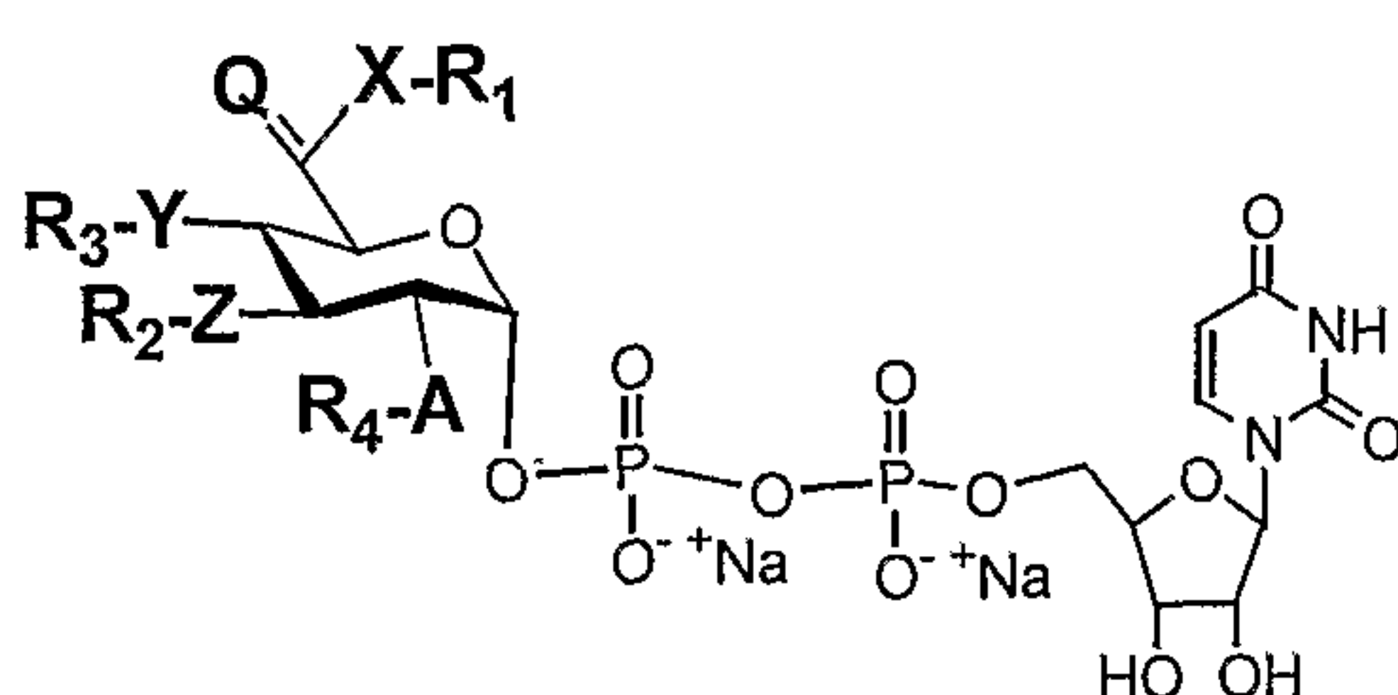
UDP-Glucose-derivatives
