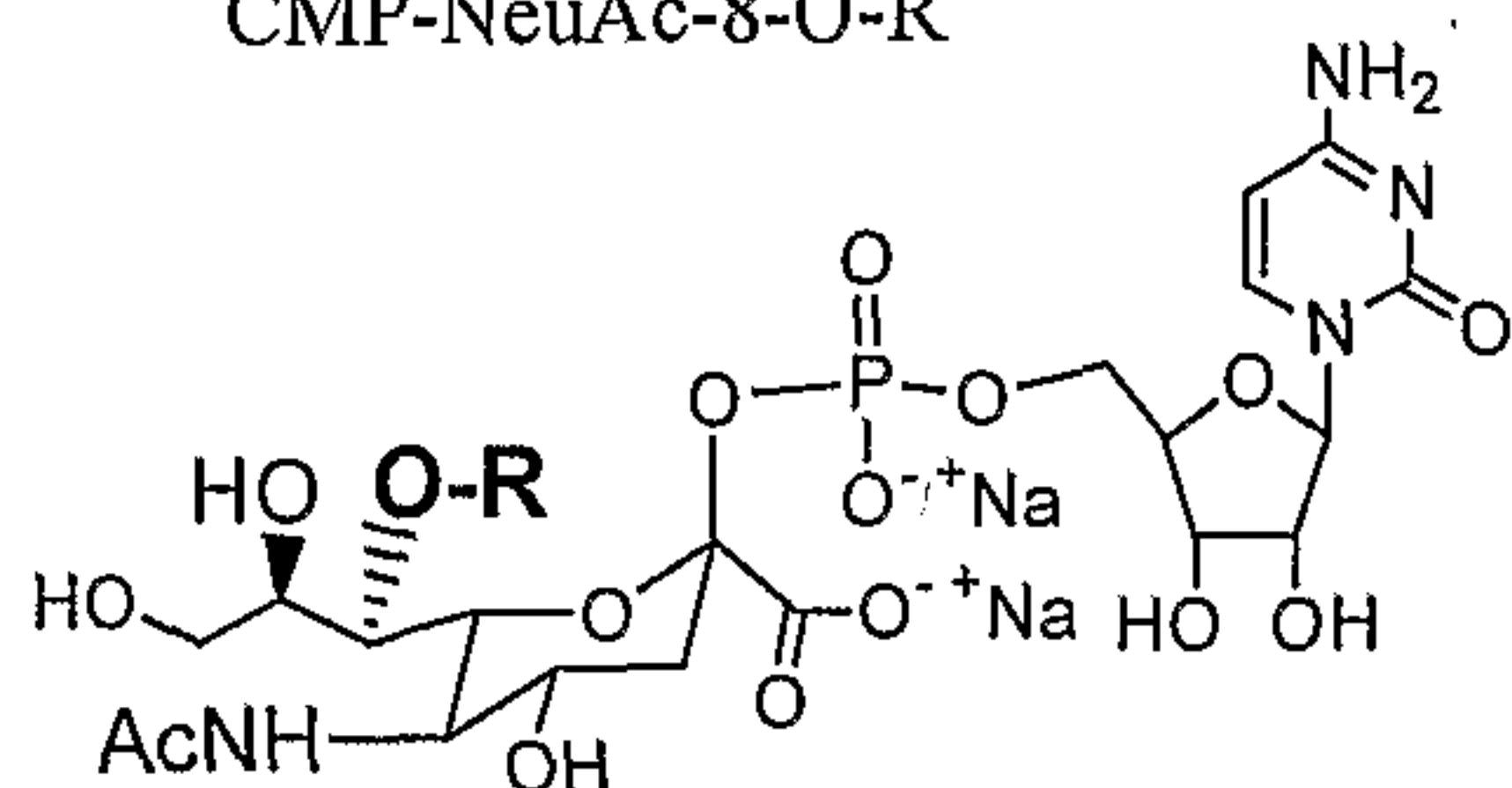
CMP-NeuAc-8-O-R
