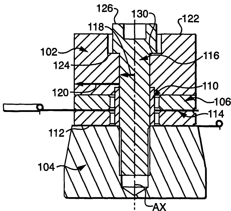
SECTION H-H
