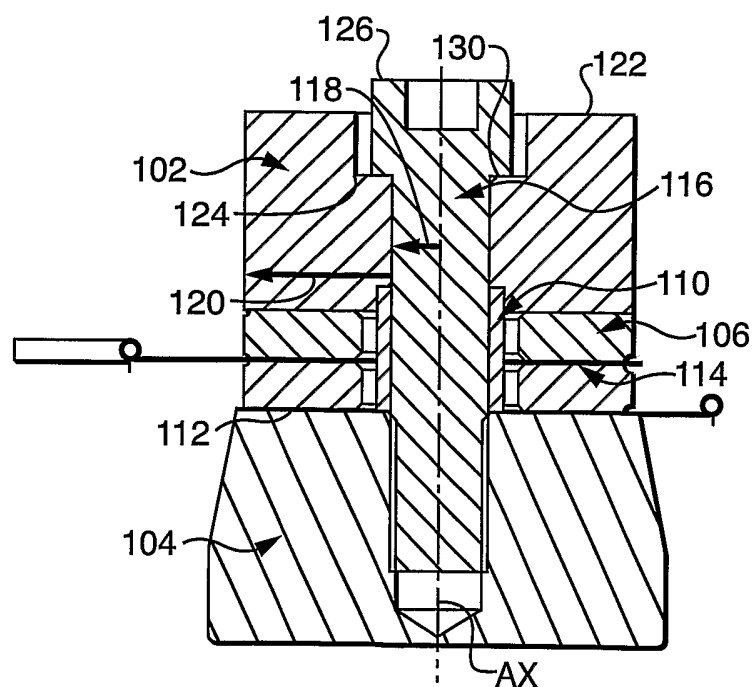
SECTION H-H
