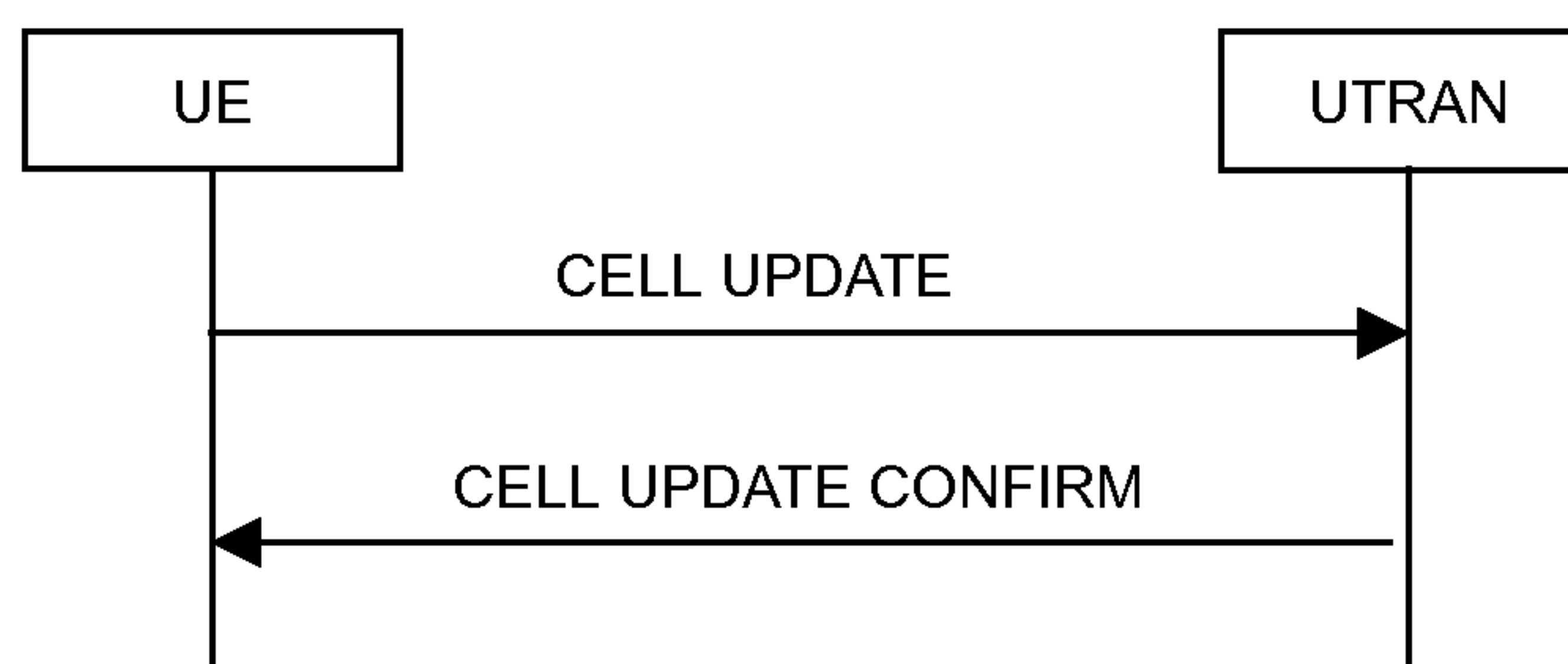
Figure 8.3.1-1: Cell update procedure, basic flow
