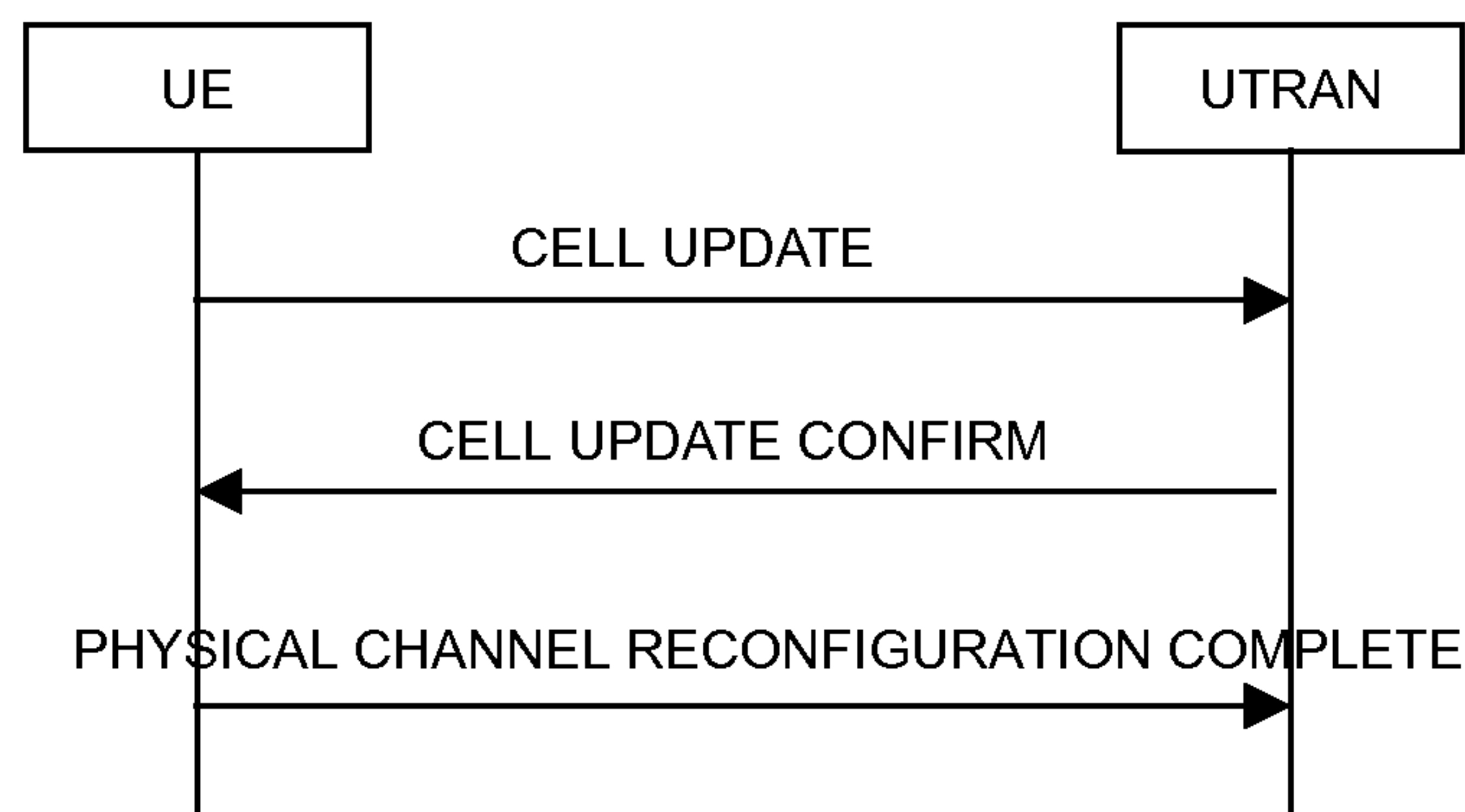
Figure 8.3.1-3: Cell update procedure with physical channel reconfiguration
