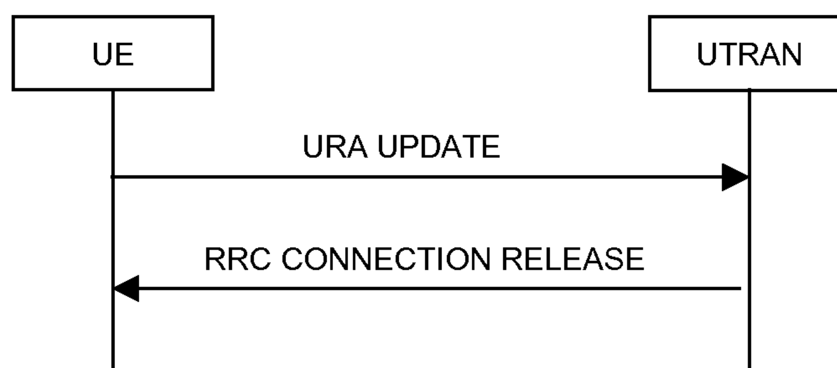
Figure 8.3.1-10: URA update procedure, failure case
