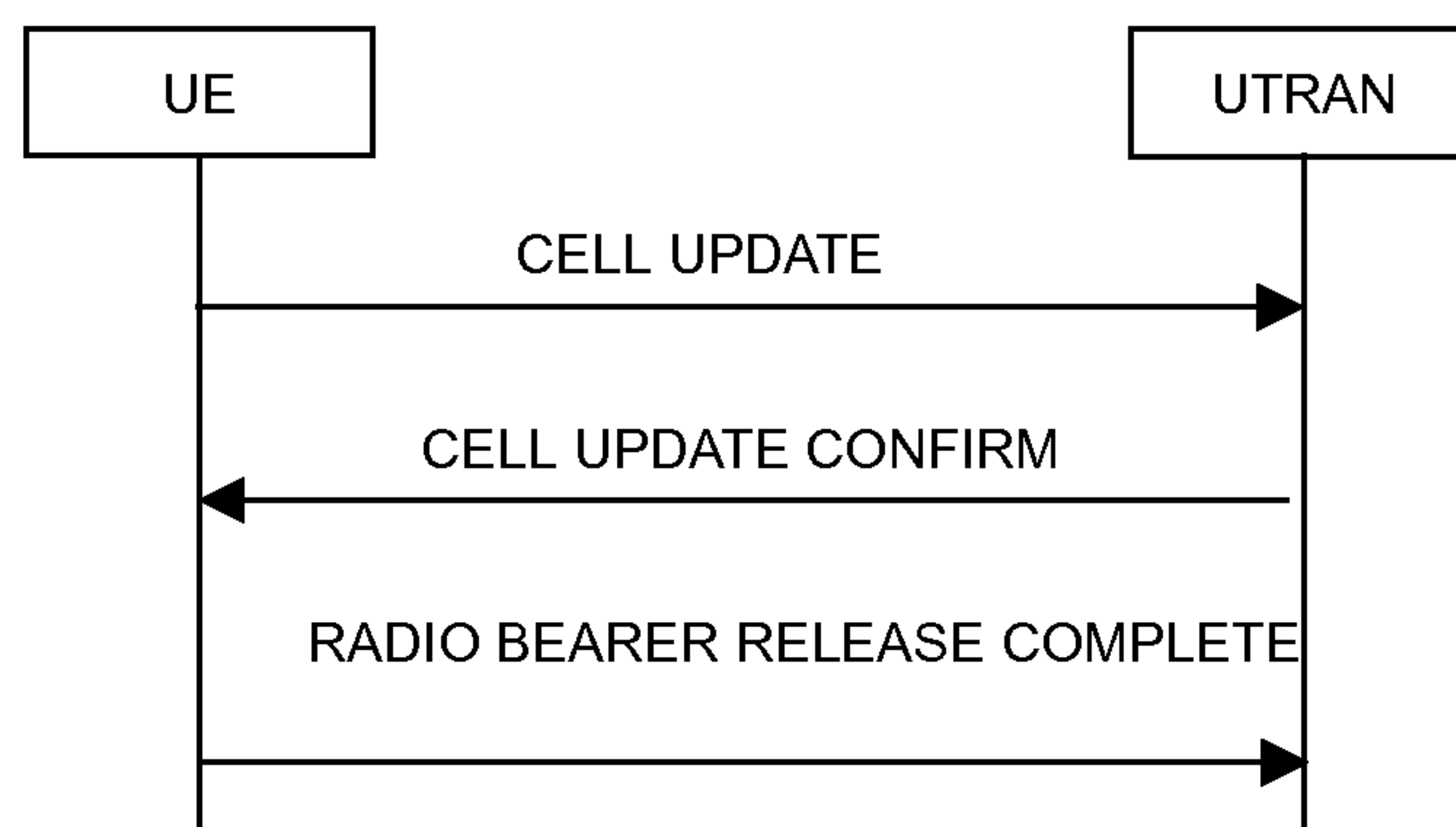
Figure 8.3.1-5: Cell update procedure with radio bearer release
