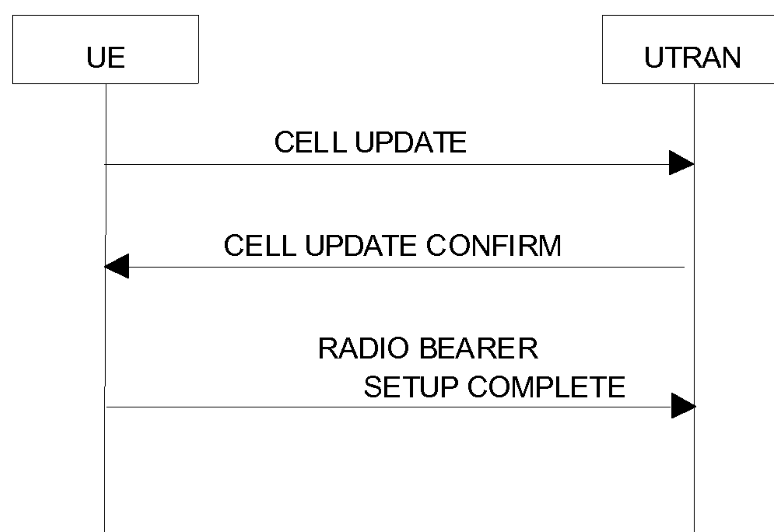
Figure 8.3.1-6a: Cell update procedure with radio bearer setup
