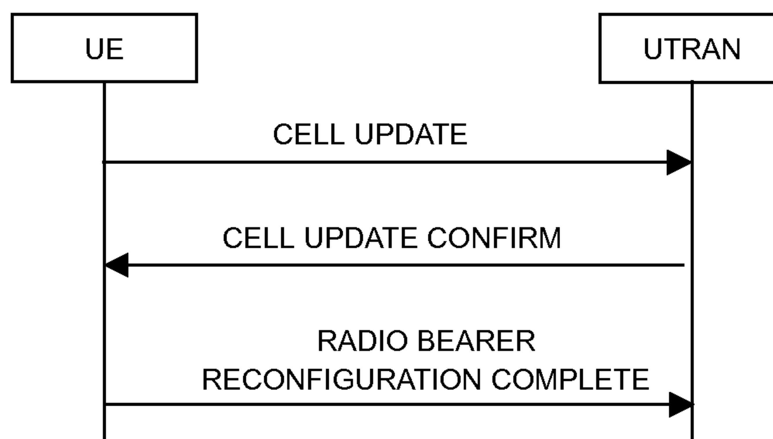
Figure 8.3.1-6: Cell update procedure with radio bearer reconfiguration
