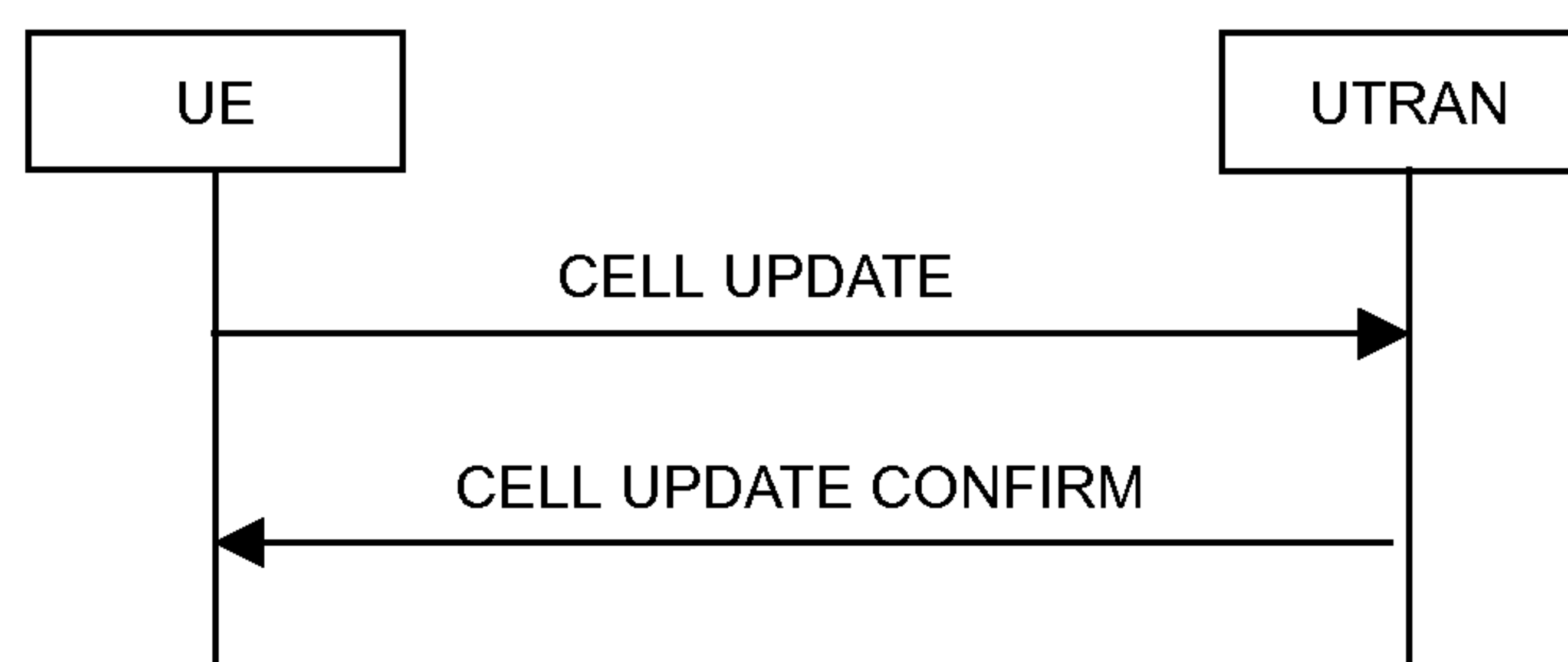
Figure 8.3.1-1: Cell update procedure, basic flow
