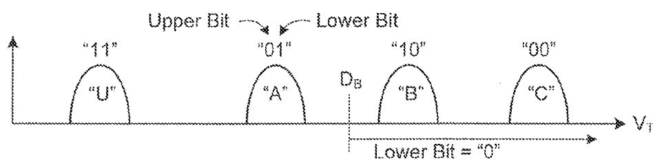
Lower Page Read (LM New Code)
