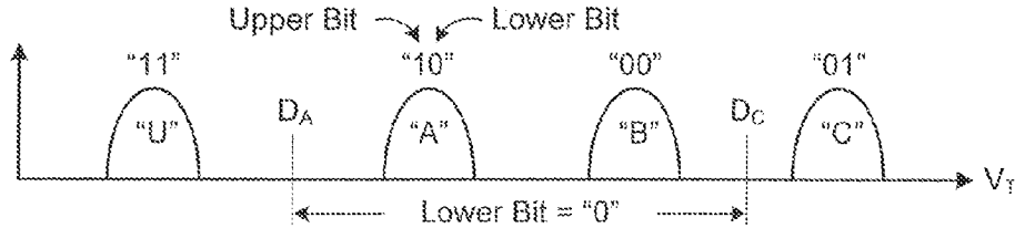
Lower Page Read (Conventional Gray Code)
