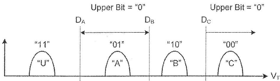
Upper Page Read (LM New Code)
