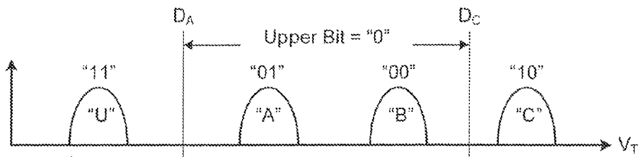
Upper Page Read (LM Gray Code)
