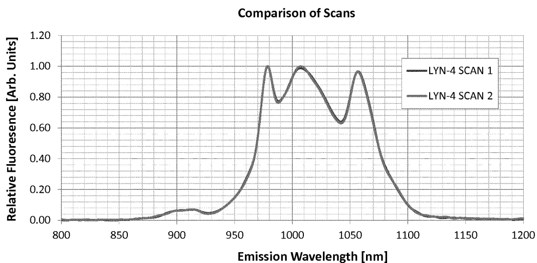
FIG. 2 LaYbNd-doped glass emission data collected at different pump energies.
