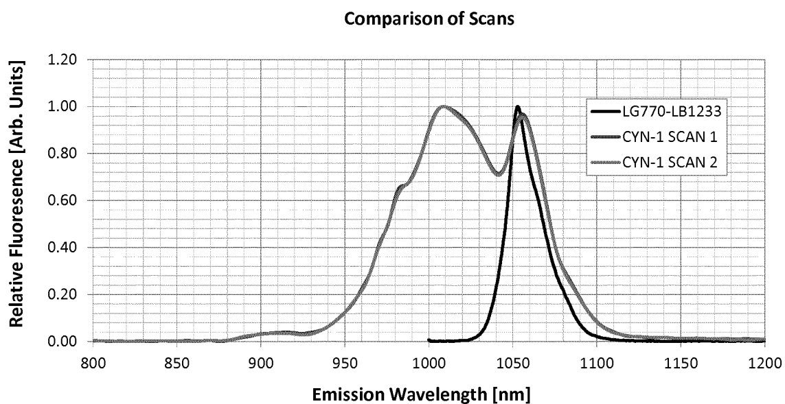
FIG. 4 Comparison of emission curves of the new ultra-broad bandwidth laser glasses containing rare earth mixture with the prior art phosphate glass, LG770.
