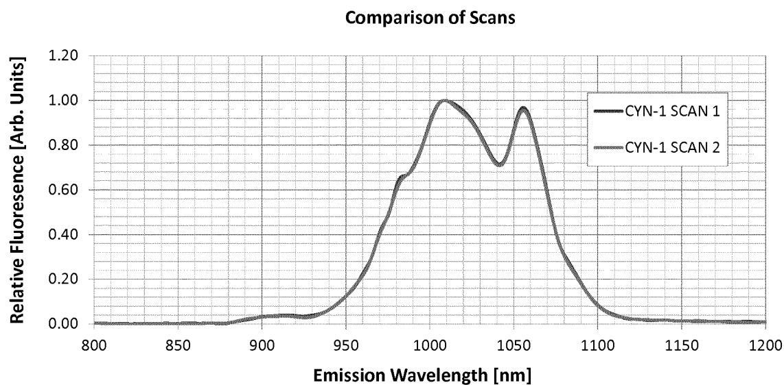
FIG. 1 Comparison of experimental emission spectra obtained at different pump energy settings for the Ce-Yb-Nd co-doped glass system.
