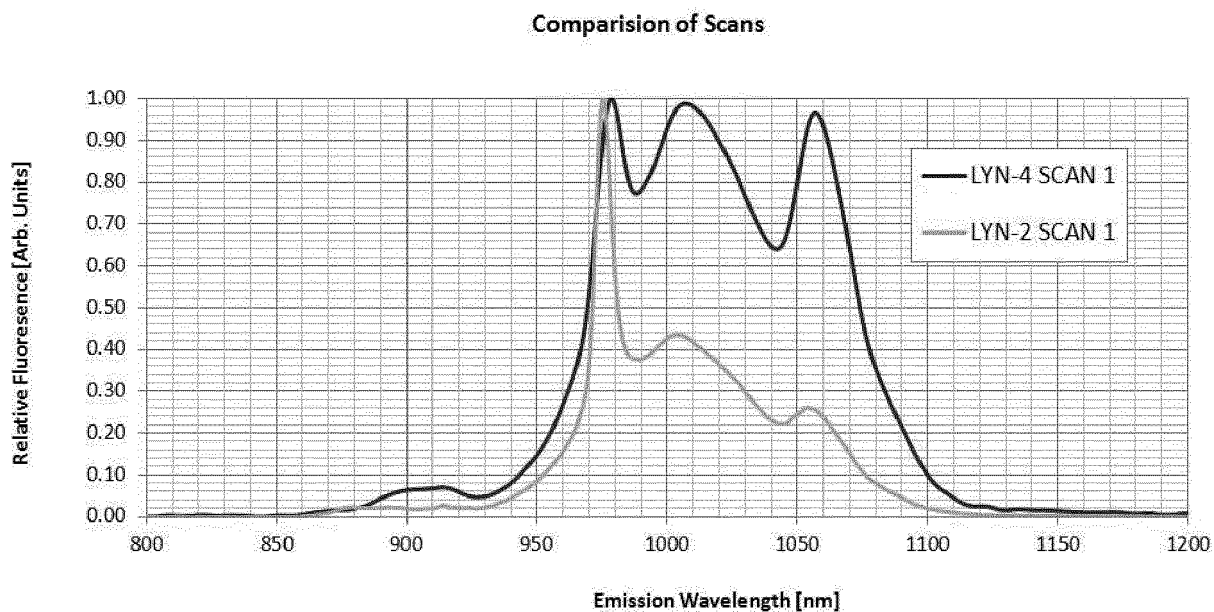
FIG. 3 Emission band-width changes as a function of dopant concentrations.
