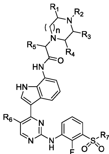
Formula (I)
