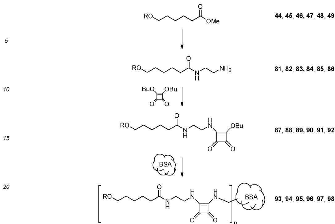
Scheme 14. Activation and conjugation of oligosaccharides 44-49 to BSA to obtain glycoconjugates 93-98 .
