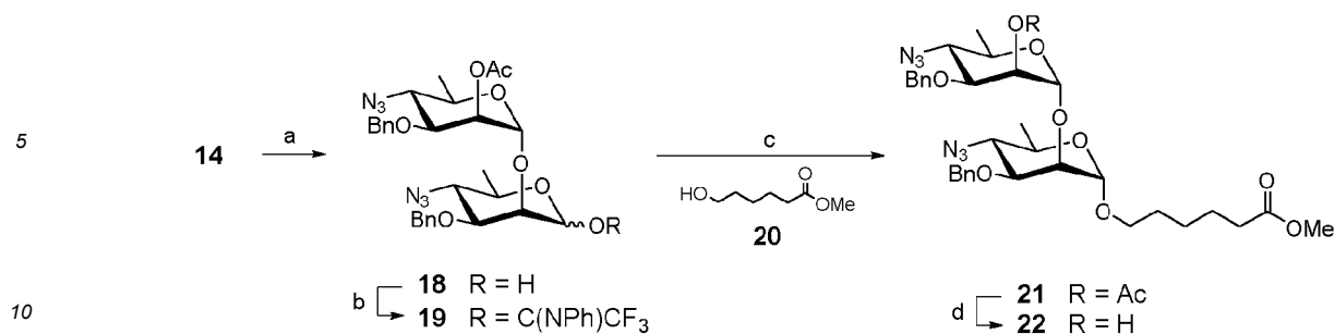
Scheme 4. a) NIS, H 2 O, acetone; b) CF 3 C(NPh)Cl, Cs 2 CO 3 , CH 2 Cl 2 ; c) TMSOTf, PhMe, 100°C; d) NaOCH 3 , CH 3 OH.
