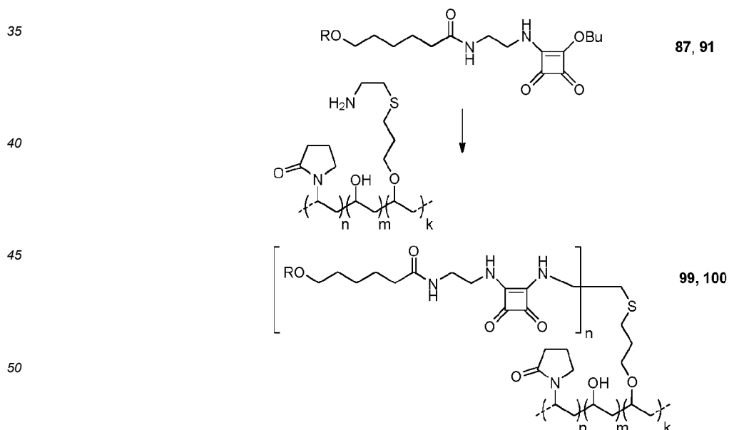
Scheme 15. Conjugation of oligosaccharides 87 and 91 to co-povidone to obtain glycoconjugates 99 and 100 .
