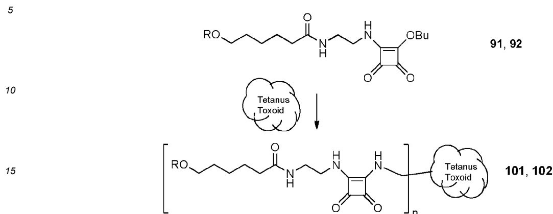
Scheme 16. Conjugation of oligosaccharides 91 and 92 to tetanus toxoid to obtain glycoconjugates 101 and 102 .
