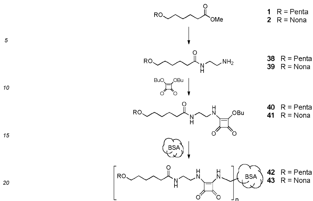
Scheme 8. Activation and conjugation of pentasaccharide 1 and nonasaccharide 2 to BSA to obtain glycoconjugates 42 and 43 .
