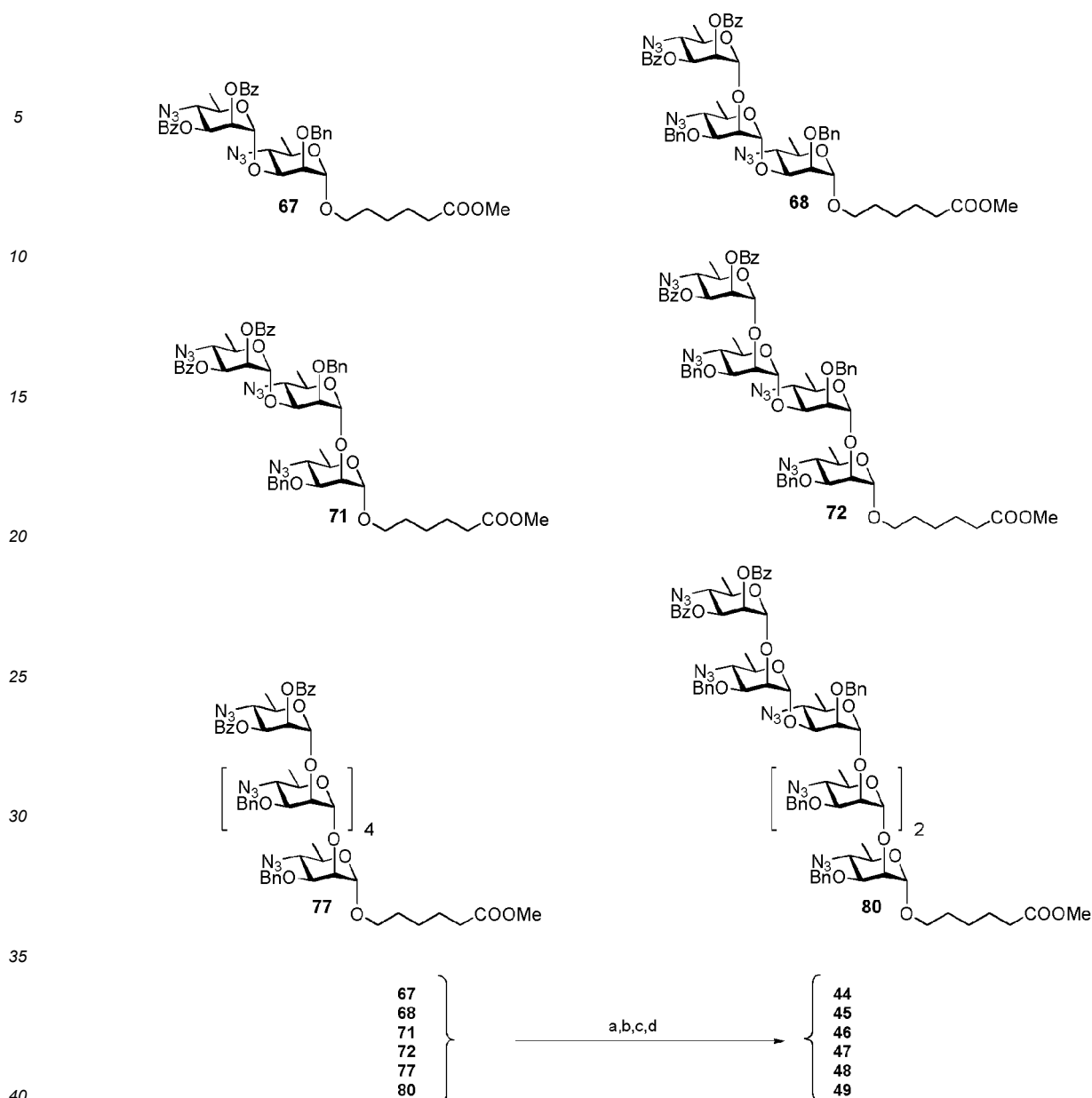
Scheme 13. a) NaOCH 3 , CH 3 OH, rt, 4 h; b) H 2 S, Py/H 2 O, 40 °C, 16 h; c) Formic anhydride, CH 3 OH, -20 °C, 3 h; d) H 2 , Pd(OH) 2 , CH 3 OH/H 2 O, rt, 16 h.
