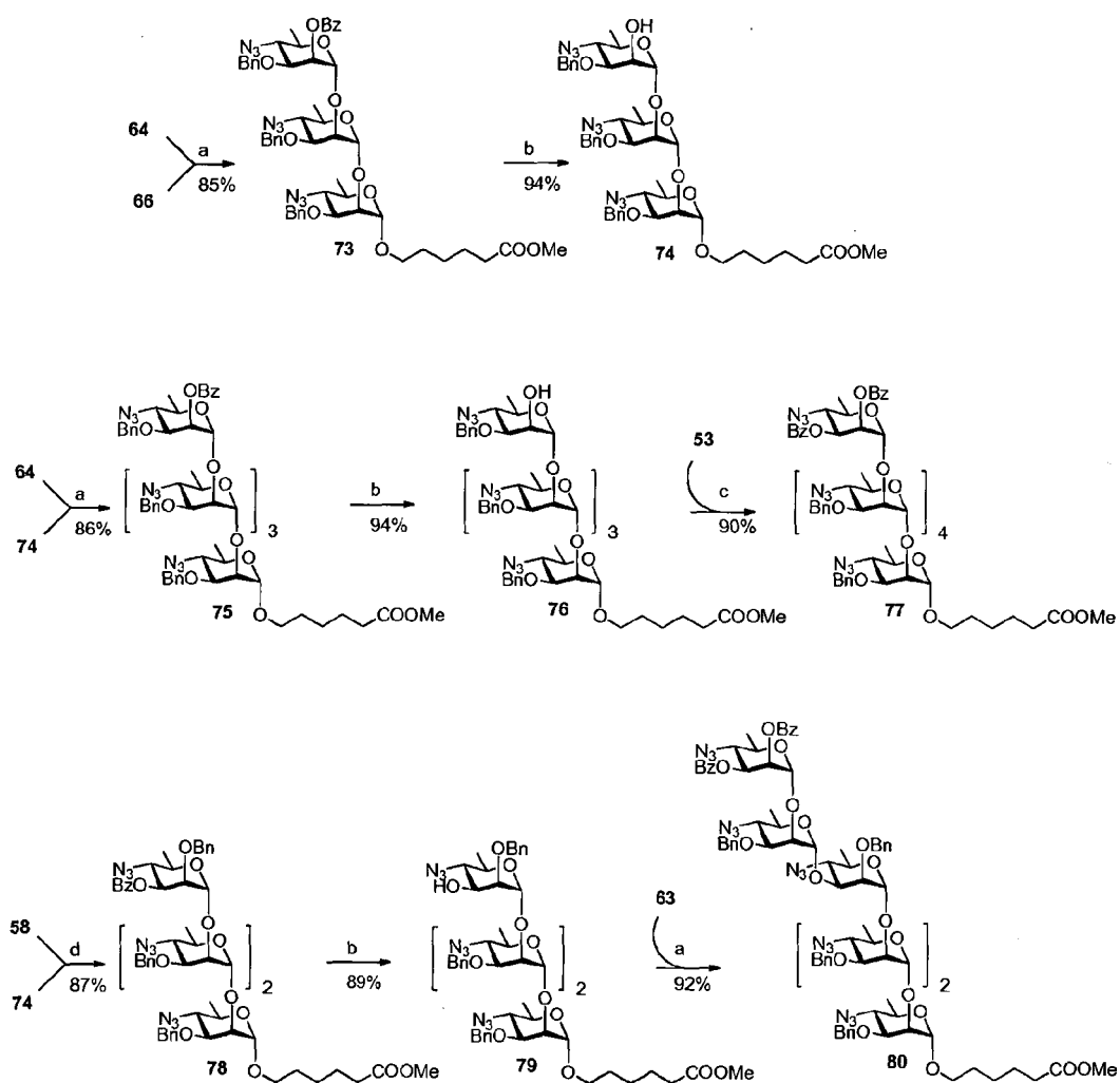
Scheme 12. a) MeOTf, 3 Å MS, CH 2 Cl 2 , rt, 48 h; b) NaOCH 3 , CH 3 OH, rt, 4 h; c) TMSOTf, 3 Å MS, CH 2 Cl 2 , rt, 1 h; d) TMSOTf, 3 Å MS, PhMe, 95 °C, 1 h.
