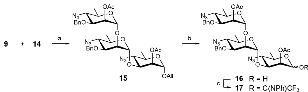
Scheme 3. a) NIS, TfOH, CH 2 Cl 2 , -30°C; b) PdCl 2 , AcONa, AcOH, H 2 O; c) CF 3 C(NPh)Cl, Cs 2 CO 3 , CH 2 Cl 2 .
