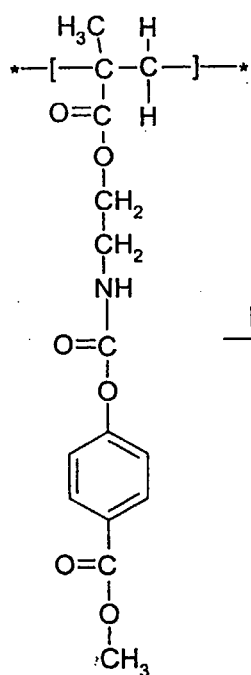
Formula 1c
