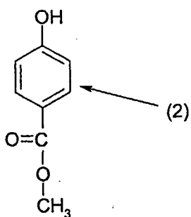
Formula 1d
