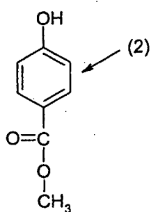
Formula 1a
