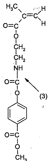
Formula 1b
