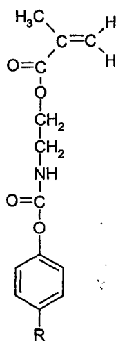
Formula 2
