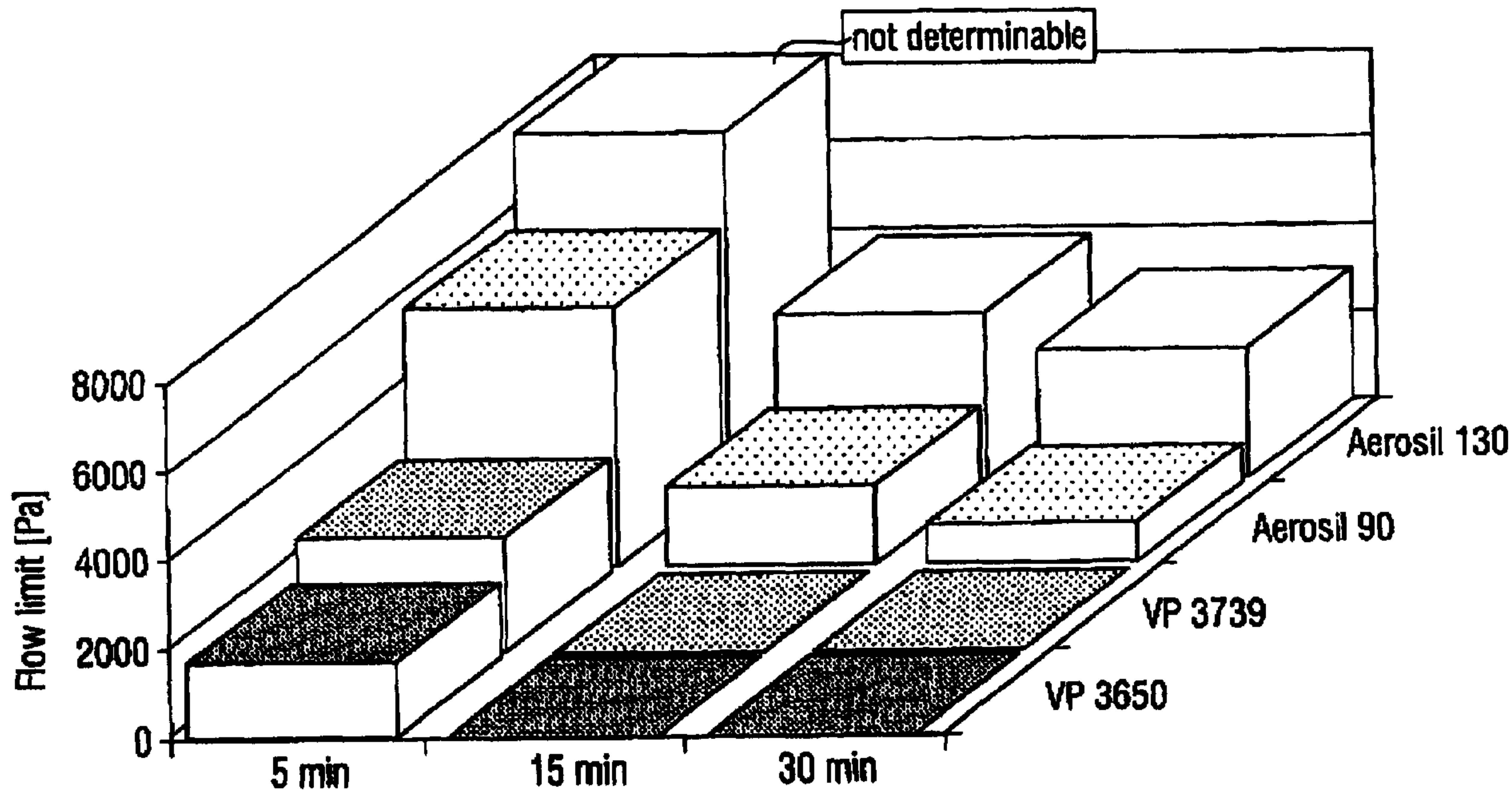
Flow limits after 5, 15, 30 minutes at the silicic acid of 20%
