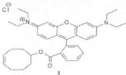
Rhodamine B-labeled cyclooctene
