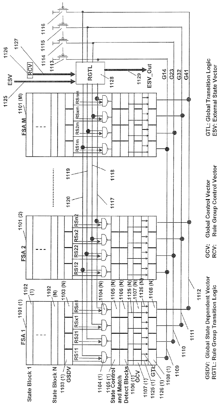
Fig. 11A PRISM Rule Group FSA Extension
