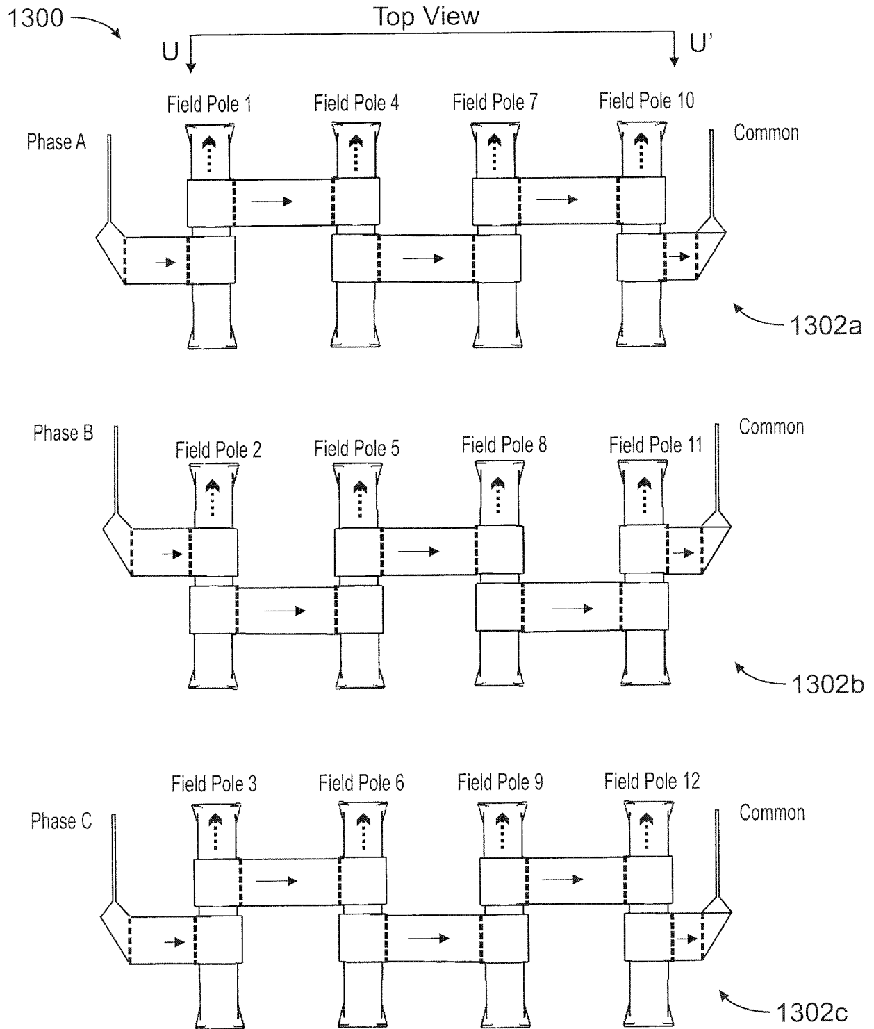
(e.g. 12 Field Pole:8 Magnet Pole Configuration)
