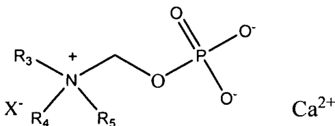
Formula V,
