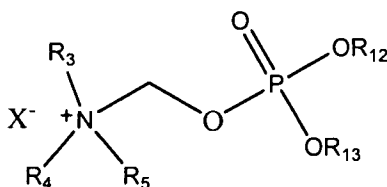
Formula VII,
