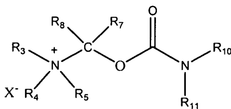
Formula VIII,
