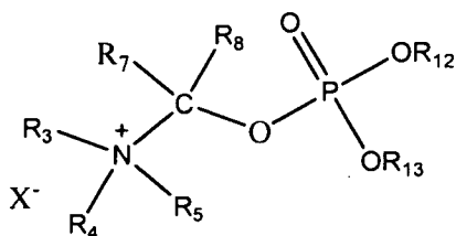
Formula VI,
