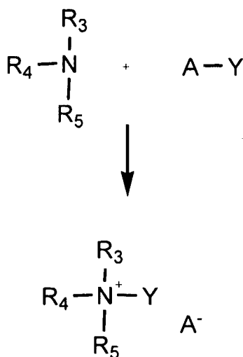
Reaction Scheme 1
