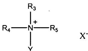
Formula III,
