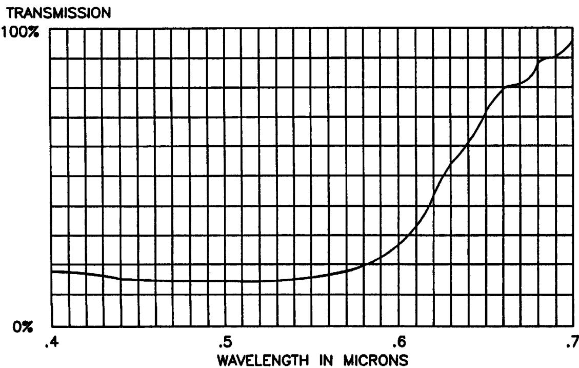
COMPLEMENTING FILTER FOR A WATER PATH OF 20 FEET
