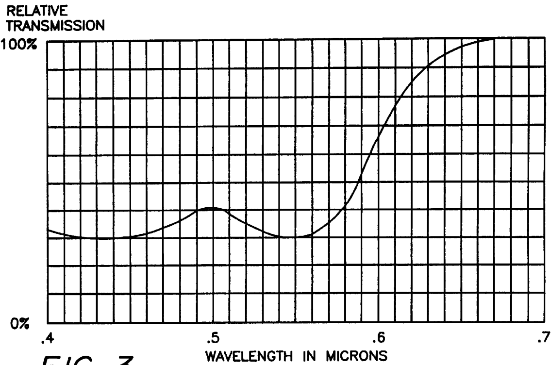
COMPLEMENTING FILTER FOR A WATER PATH OF 5 FEET
