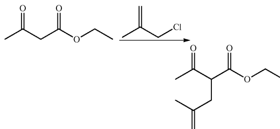
Ethyl 2-acetyl-4-methylpent-4-enoate
