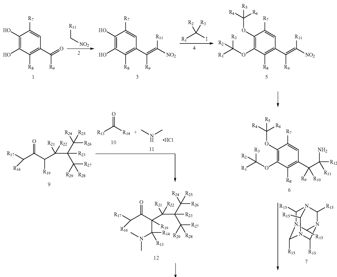
Scheme I
