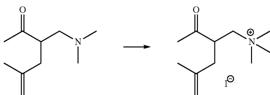
2-Acetyl-N,N,N,4-tetramethylpent-4-en-1-aminium iodide
