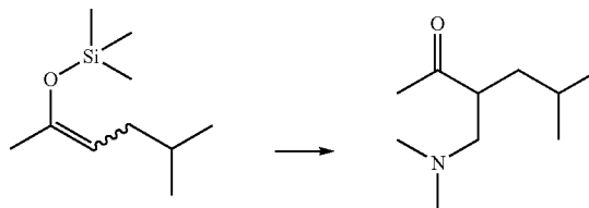
3-[(Dimethylamino)methyl]-5-methylhexan-2-one
