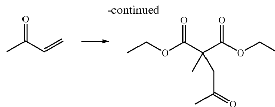
1,3-Diethyl 2-methyl-2-(3-oxobutyl)propanedioate
