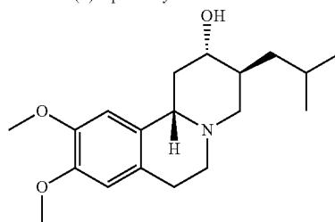
(-)-alpha-dihydrotetrabenzazine
