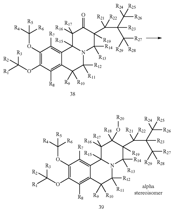
Scheme VIII
