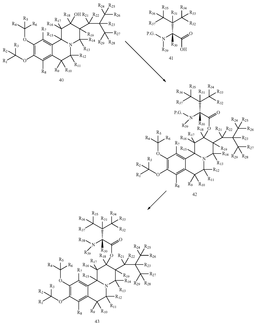
Scheme X
