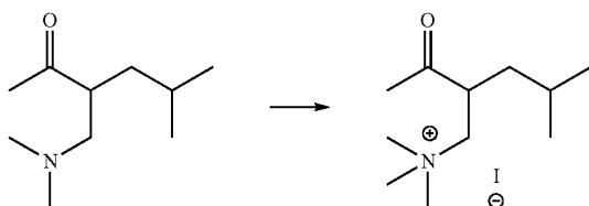
2-Acetyl-N,N,N,4-tetramethylpentan-1-aminium iodide
