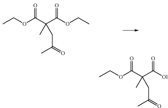
2-(Ethoxycarbonyl)-2-methyl-5-oxohexanoic acid
