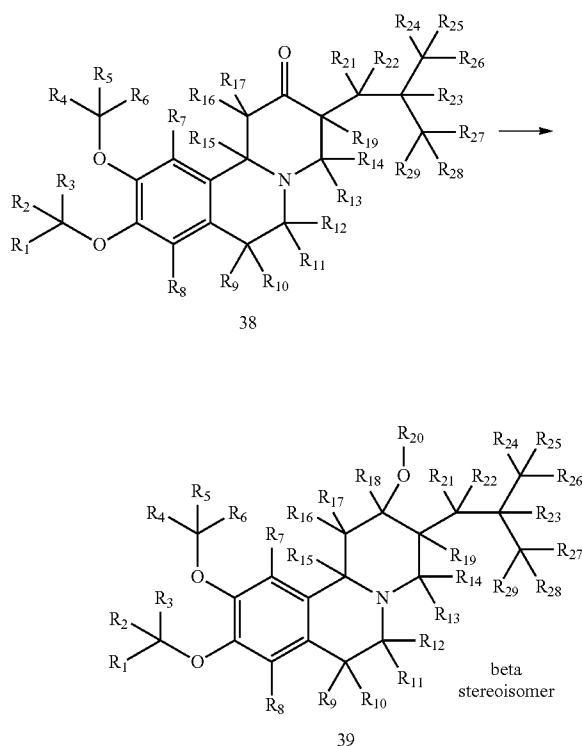
Scheme IX
