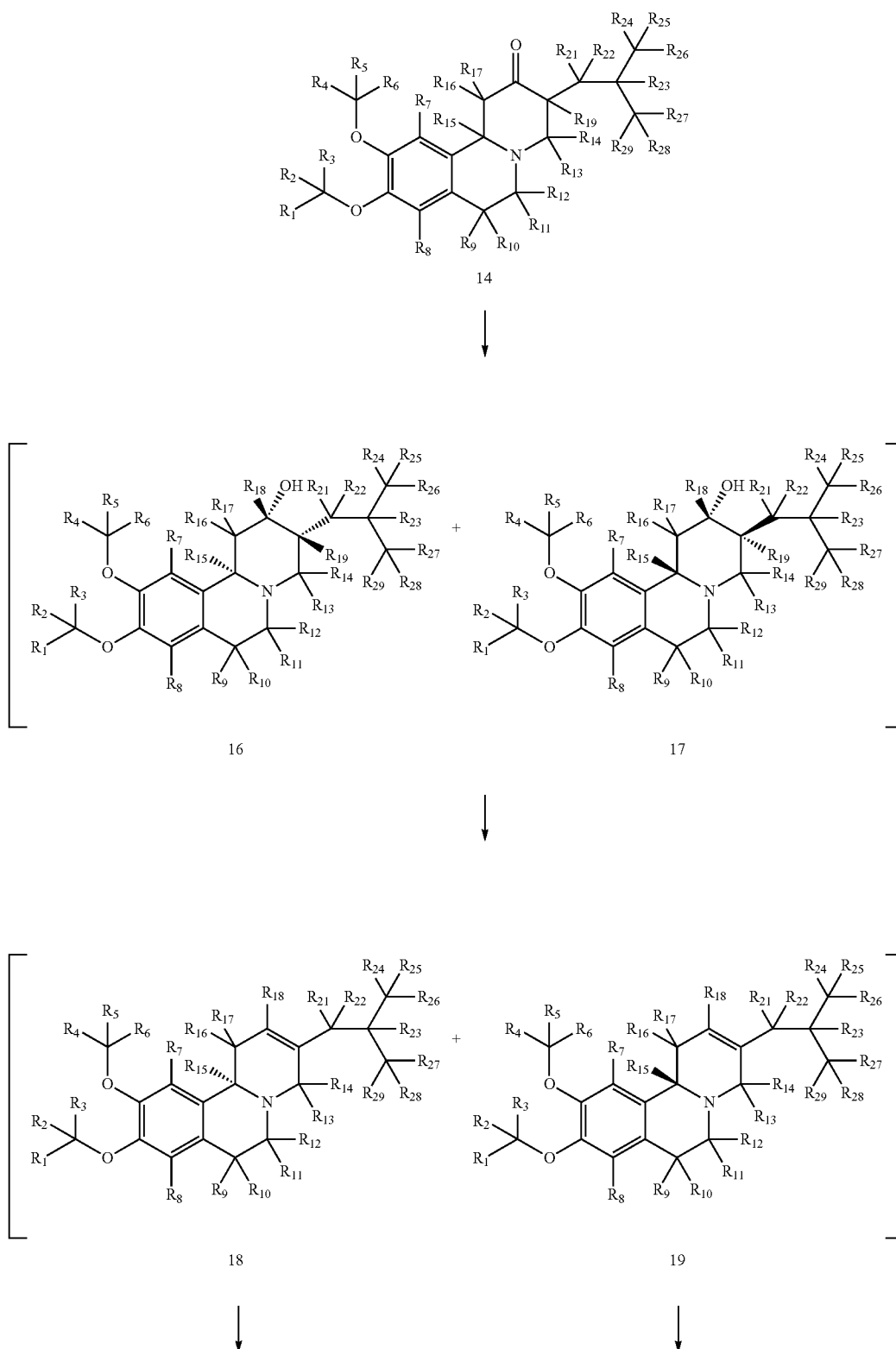
Scheme II
