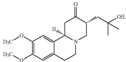
(3R, 11bR)-enantiomer
