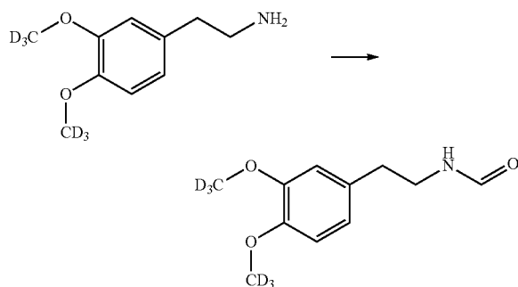
D 6 -N-[2-(3,4-dimethoxyphenyl)ethyl]formamide
