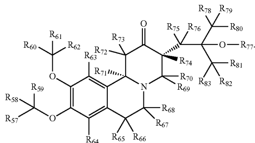
(3R, 11bR)-enantiomer
