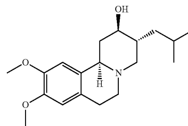
(+)-alpha-dihydrotetrabenzazine
