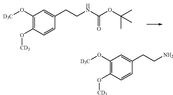
D 6 -2-(3,4-dimethoxyphenyl)ethanamine
