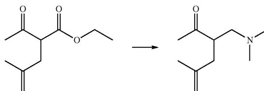
3-((Dimethylamino)methyl)-5-methylhex-5-en-2-one
