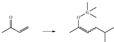
Trimethyl(5-methylhex-2-en-2-yloxy)silane
