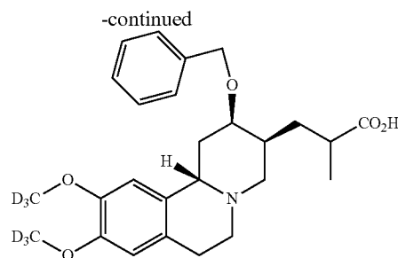
D_6 -2-(benzyloxy)-9,10-dimethoxy-2,3,4,6,7,11b-hexahydro-1H-pyrido[2,1-a]isoquinolin-3-yl)-2-methylpropanoic acid (mixture of diastereomers)
