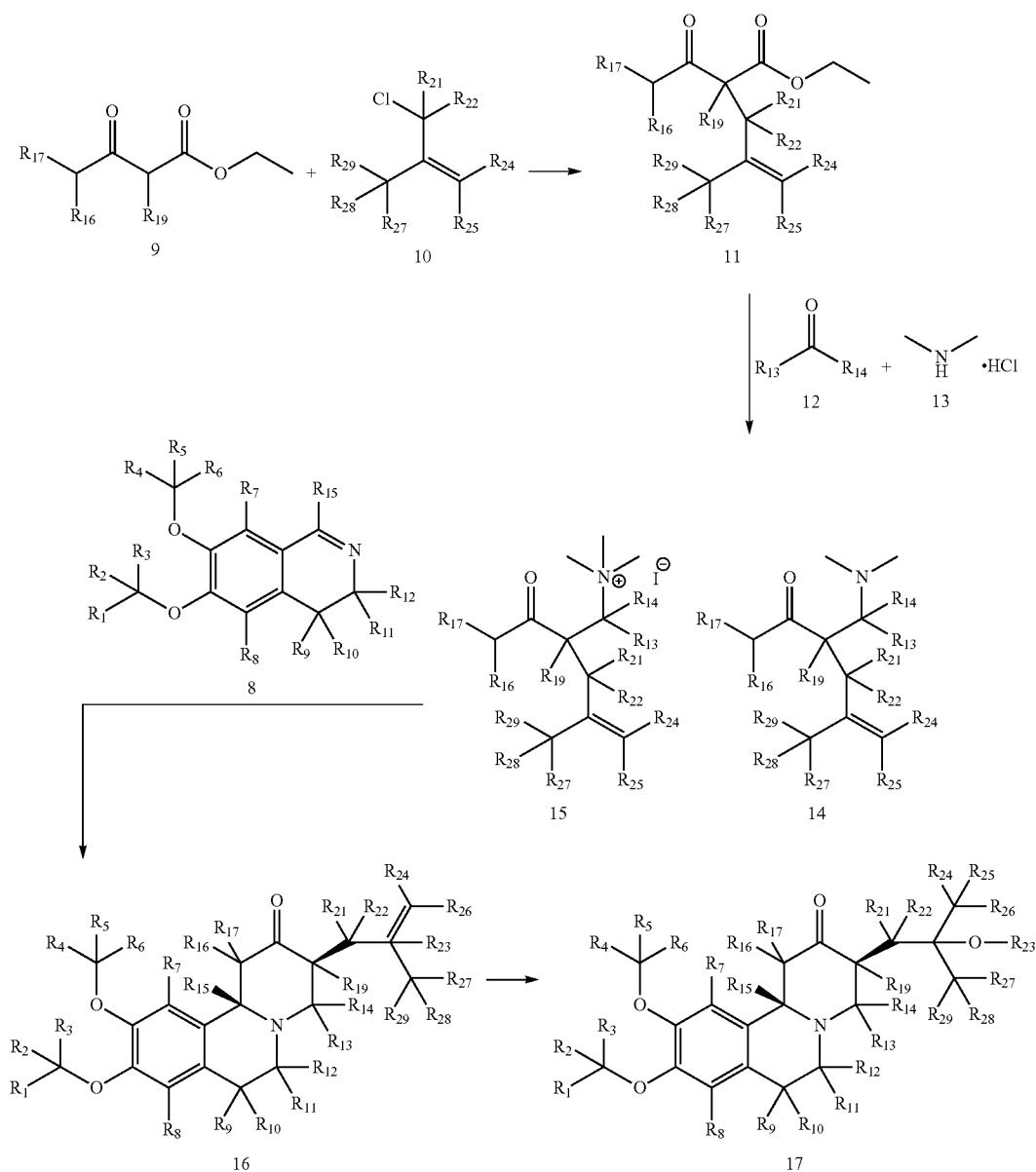
Scheme XI
