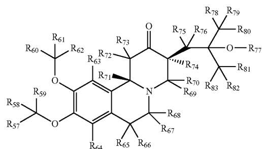
(3S, 11bS)-enantiomer
