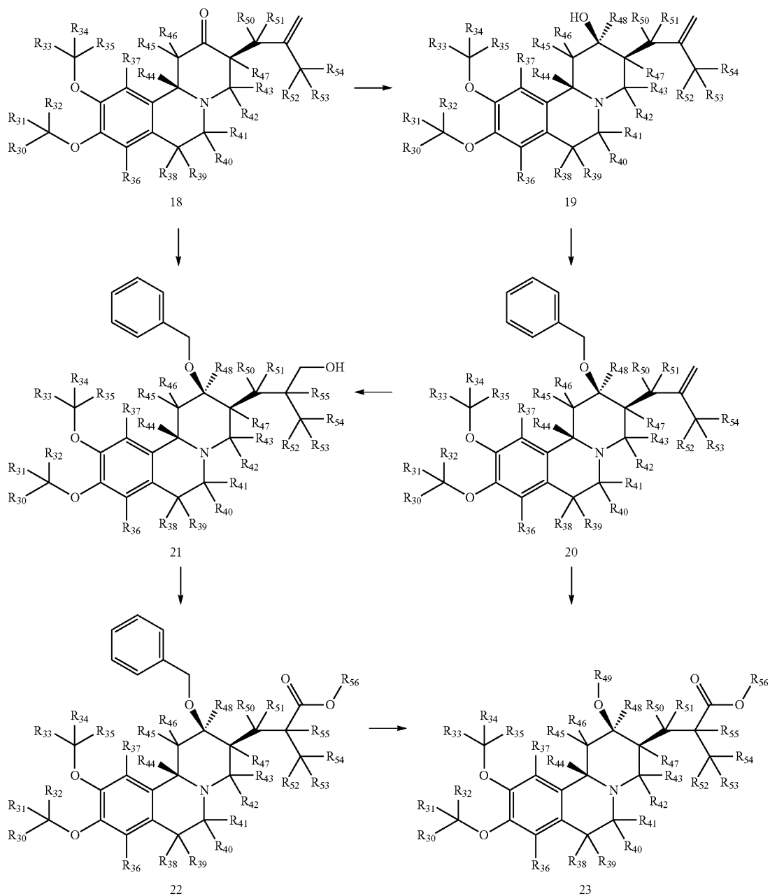
Scheme XII
