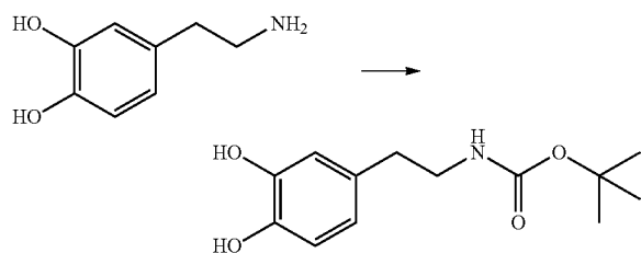
Tert-butyl 3,4-dihydroxyphenethylcarbamate
