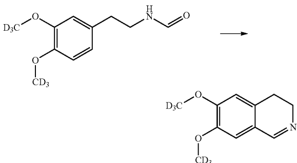
D_6 -6,7-dimethoxy-3,4-dihydroisoquinoline
