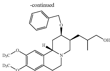
D_6 -2-(benzyloxy)-9,10-dimethoxy-2,3,4,6,7,11b-hexahydro-1H-pyrido[2,1-a]isoquinolin-3-yl)-2-methylpropan-1-ol (mixture of diastereomers)
