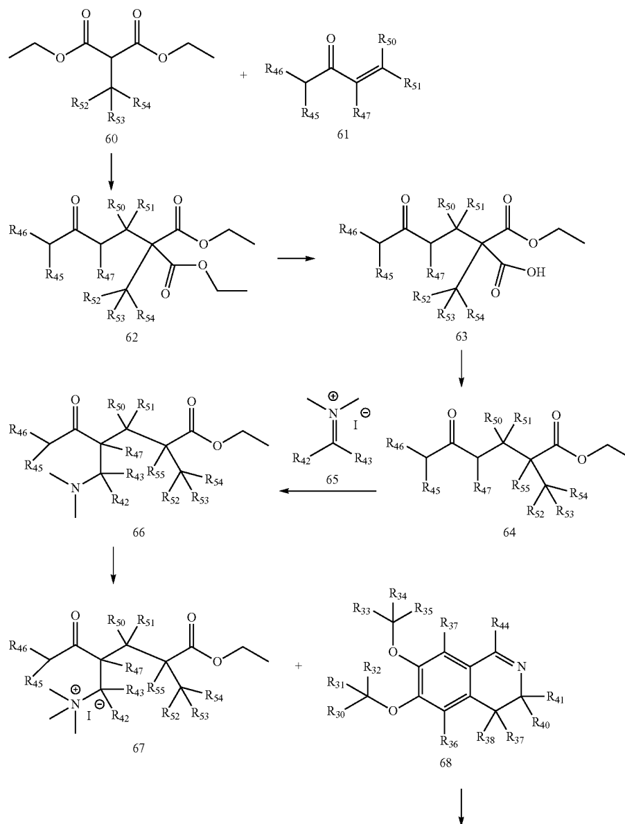
Scheme XIII
