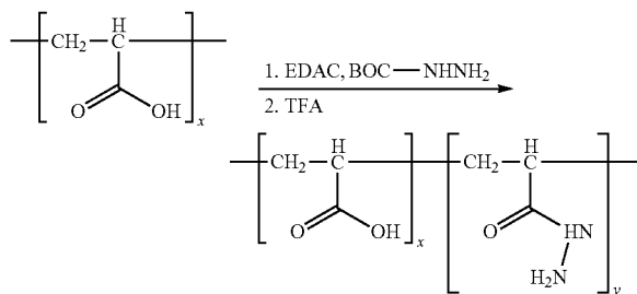
Scheme 4 Polyacrylic Acid Synthesis
