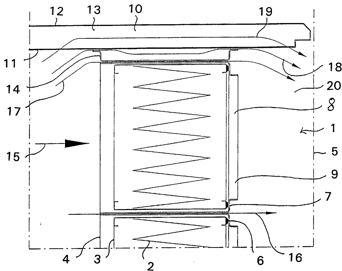
Fig. 1 Prior Art
