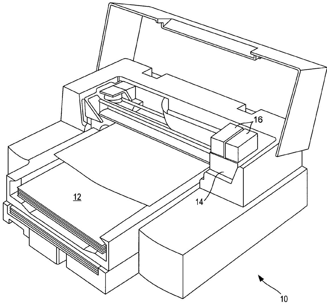
FIG. 1 (Background Art)
